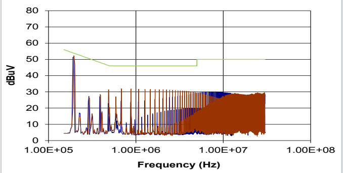
NXJ2S2415MC (Average)
