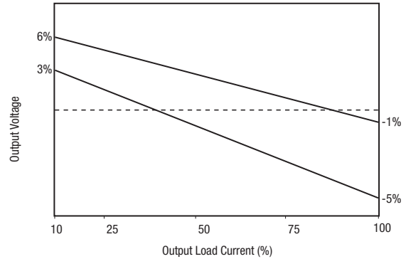
NXJ2S2405MC
