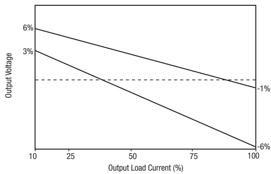
NXJ2S2415MC
