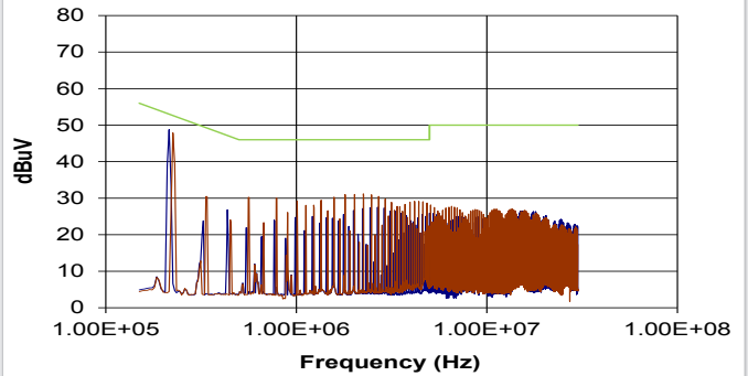
NXJ2S2405MC (Average)
