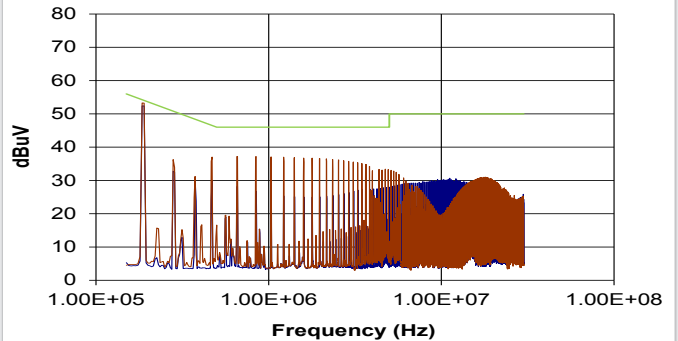
NXJ2S2415MC (Average)
