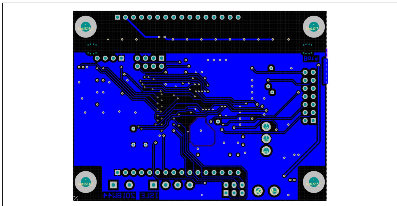
Figure 57 View of control PCB bottom layer
