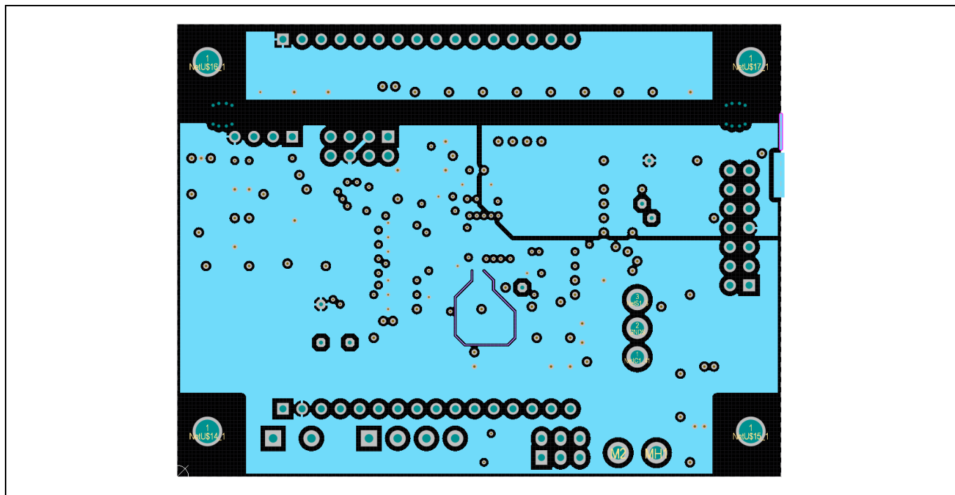
Figure 56 View of control PCB inner 2 layer
