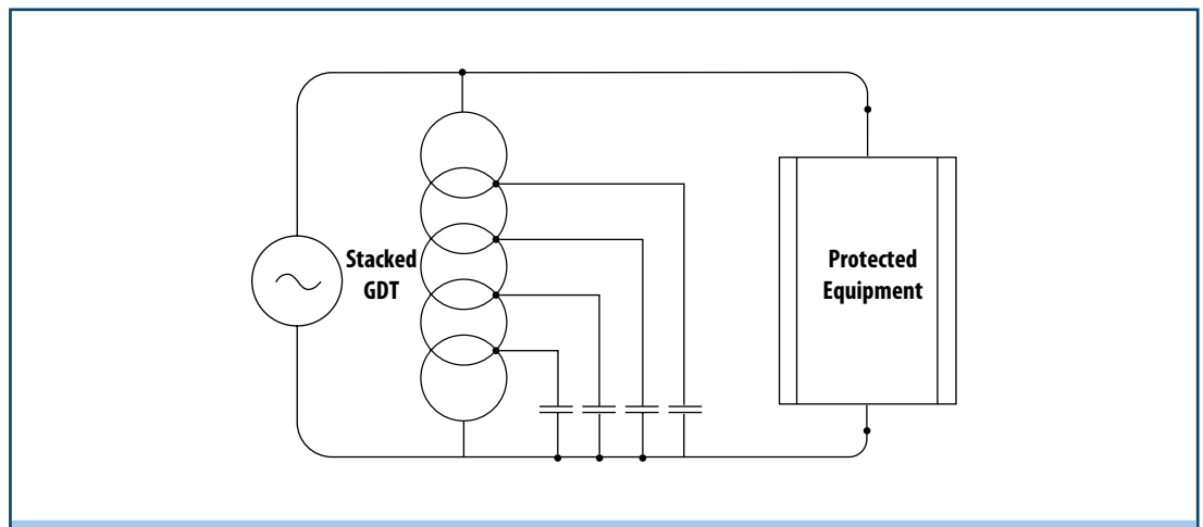
Figure 3. | Schematic illustrating the use of a Stacked GDT
