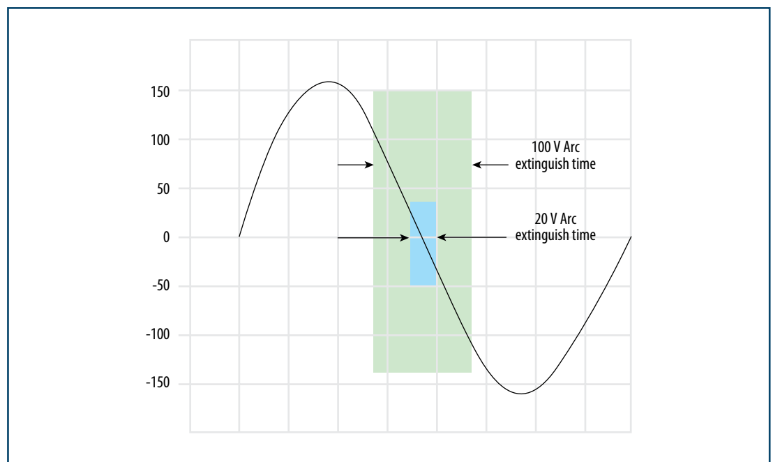
Figure 4. | Arc extinguishing times: 20 V vs. 100 V
