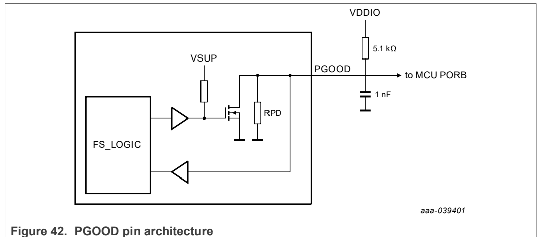
Figure 42. PGOOD pin architecture
