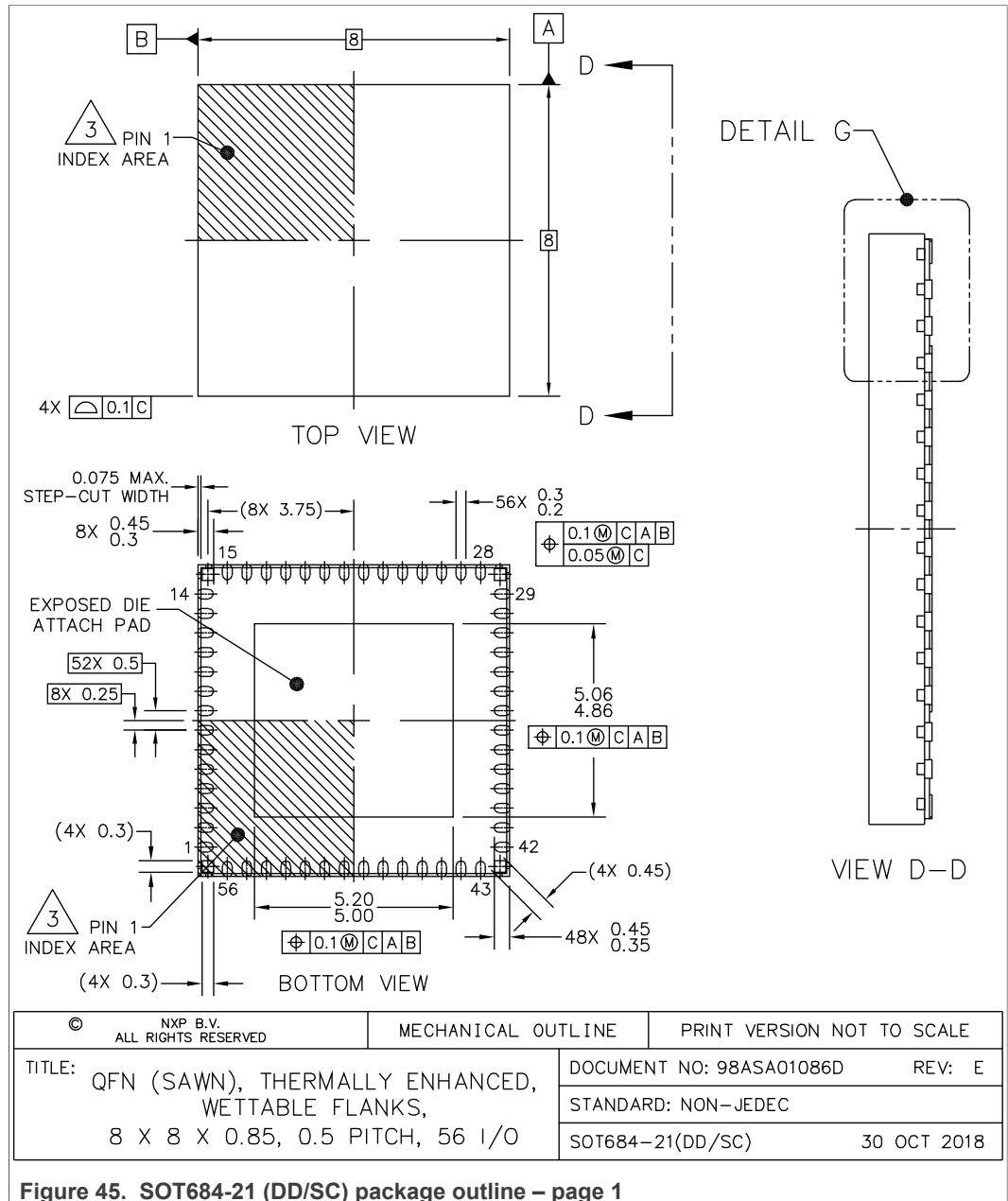
Figure 45. SOT684-21 (DD/SC) package outline – page 1
