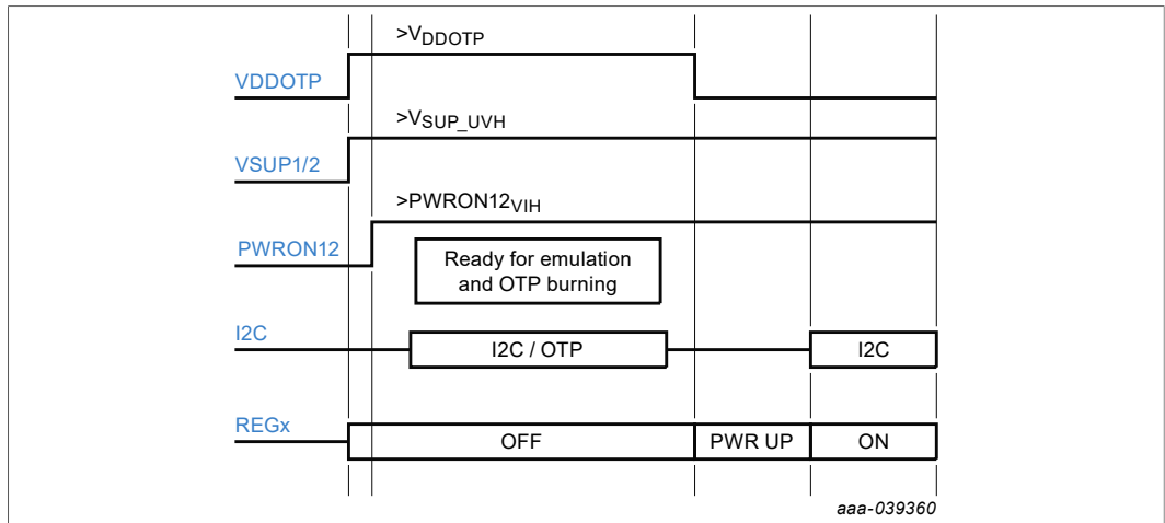
Figure 8. Debug mode entry
