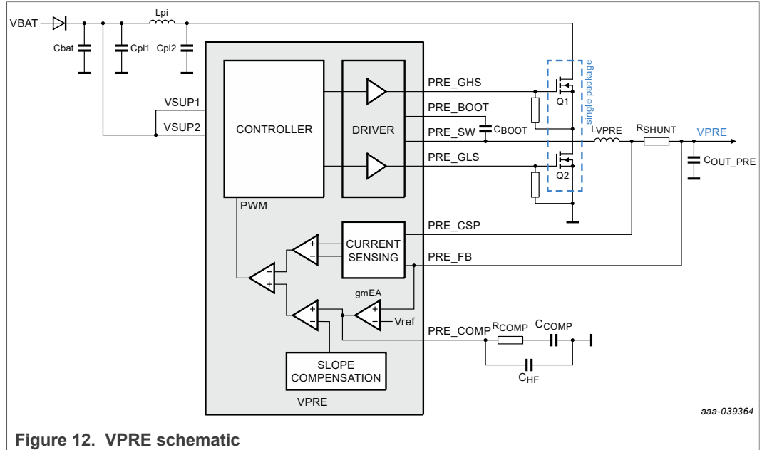
Figure 12. VPRES schematic
