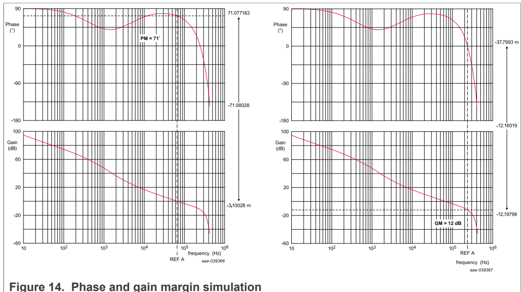
Figure 14. Phase and gain margin simulation
