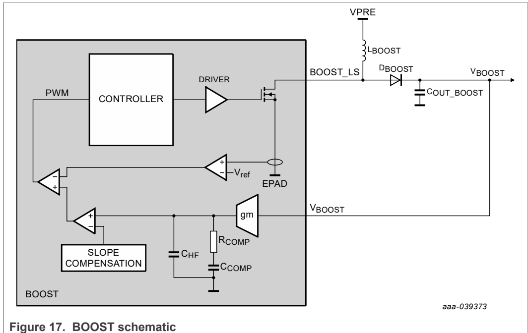
Figure 17. BOOST schematic
