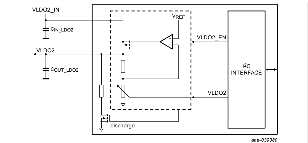
Figure 22. LDO2 block diagram
