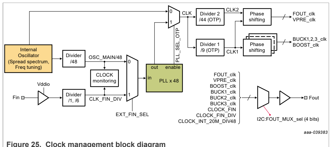
Figure 25. Clock management block diagram
