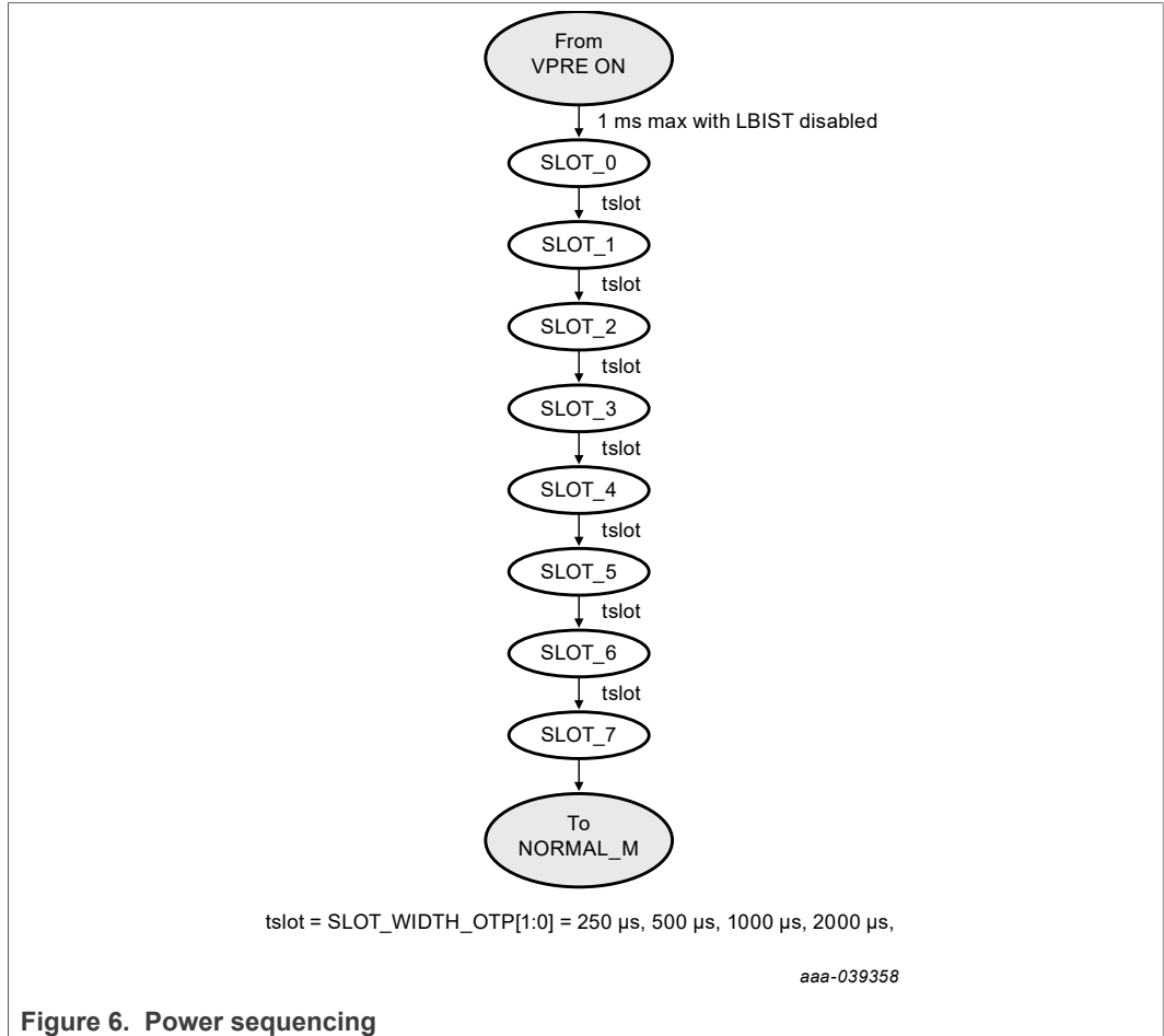
Figure 6. Power sequencing
