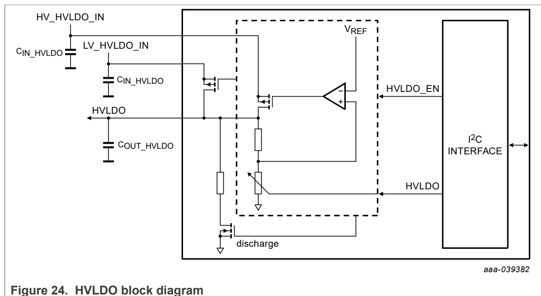
Figure 24. HVLDO block diagram
