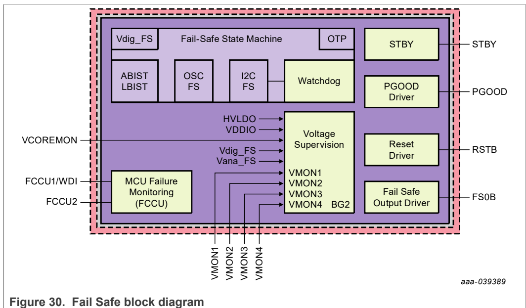
Figure 30. Fail Safe block diagram
