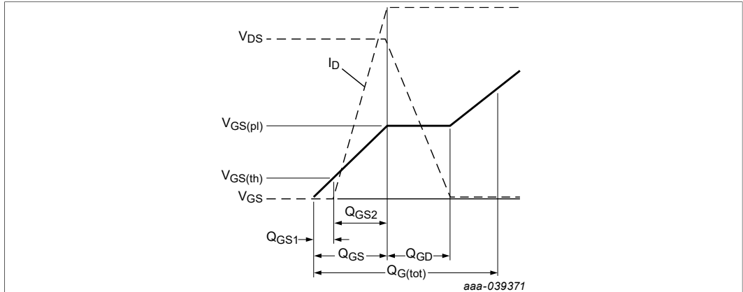
Figure 16. MOSFET gate charge definition
