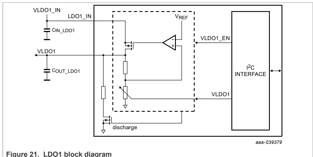
Figure 21. LDO1 block diagram
