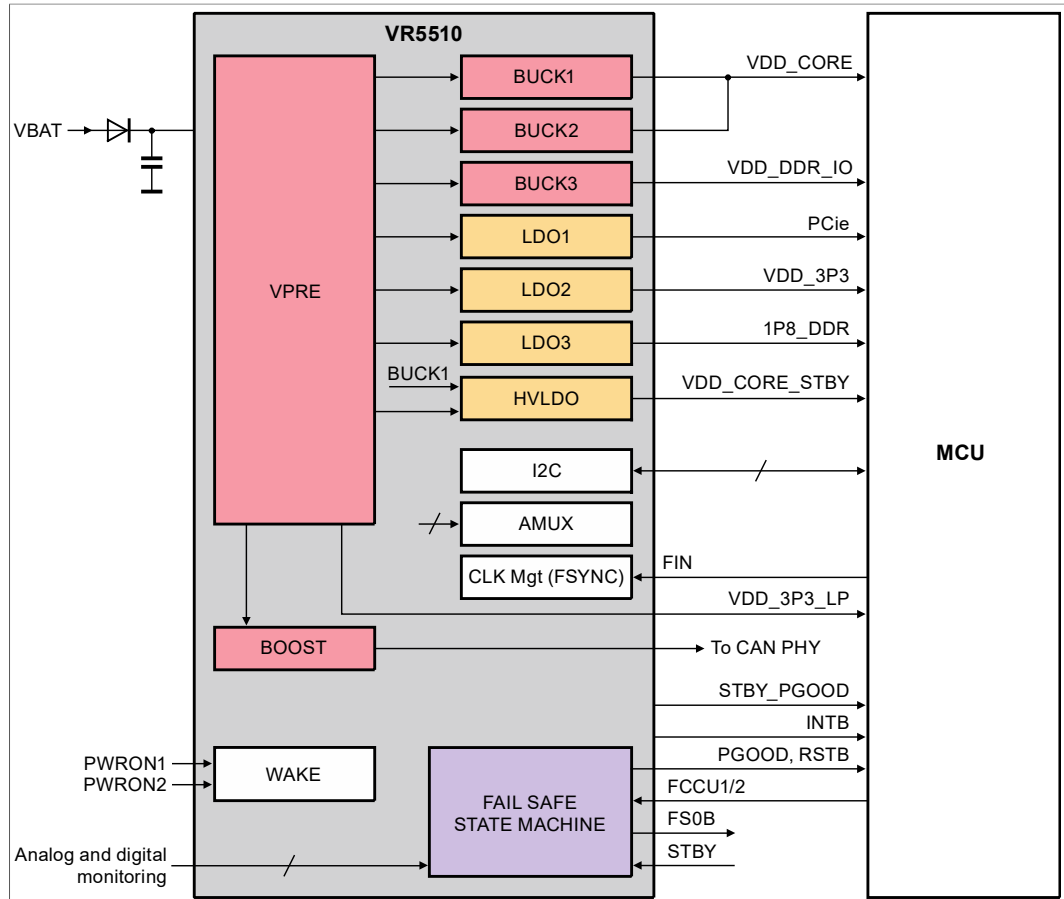
Figure 1. VR5510 simplified application diagram
