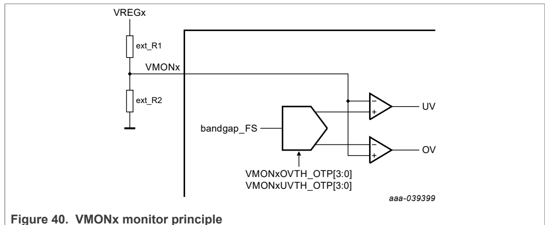
Figure 40. VMONx monitor principle
