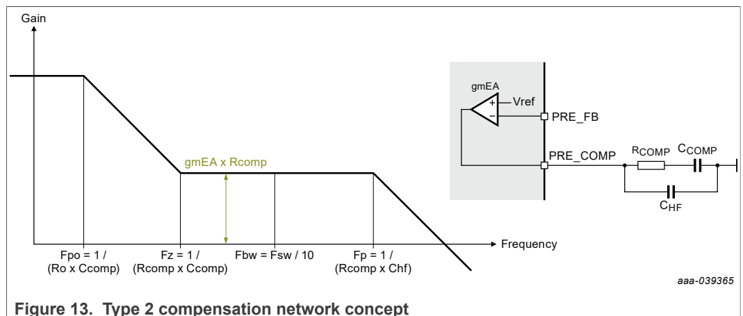
Figure 13. Type 2 compensation network concept
