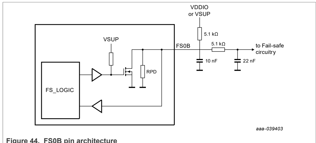
Figure 44. FS0B pin architecture
