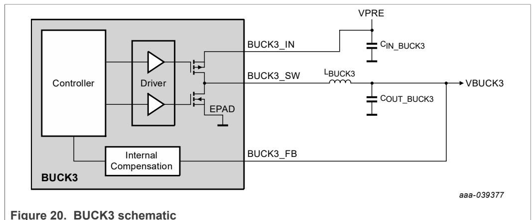
Figure 20. BUCK3 schematic
