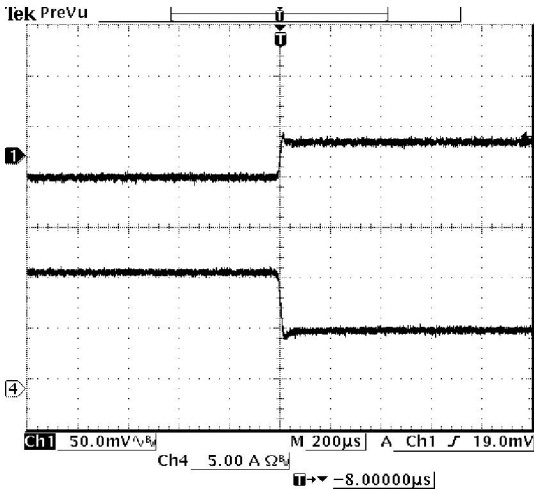
100%-50% Load Transients at Vin=12V, Vout=0.6V@Ta=25°C
