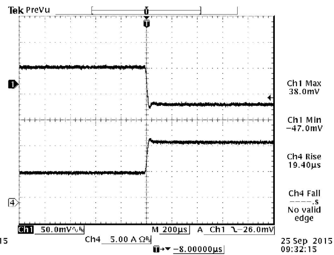
50%-100% Load Transients at Vin=12V, Vout=3.3V@Ta=25°C
