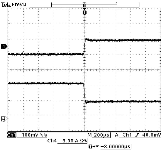
100%-50% Load Transients at V_{in}=12V , V_{out}=5.5V@T_a=25^{\circ}C
