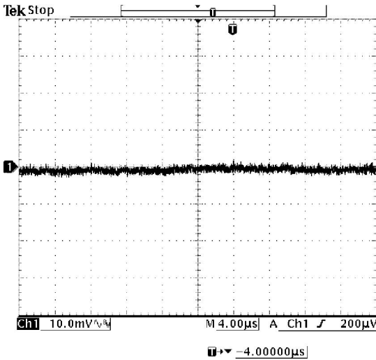
Ripple and noise at full load, 12V input, 0.6V output and Ta=25 degC
