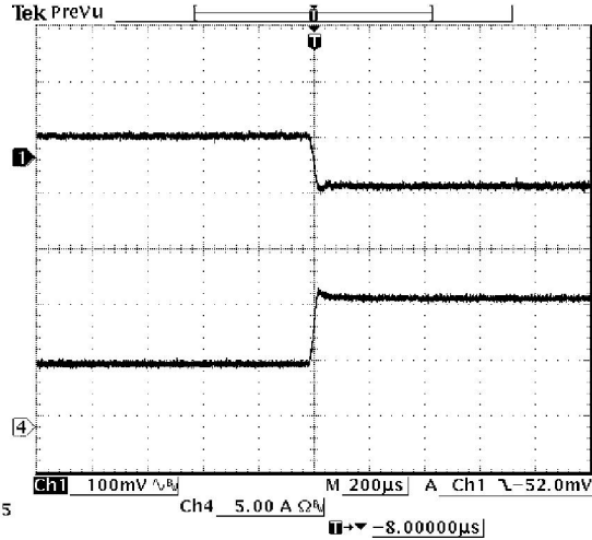
50%-100% Load Transients at V_{in}=12V , V_{out}=5.5V@T_a=25^{\circ}C
