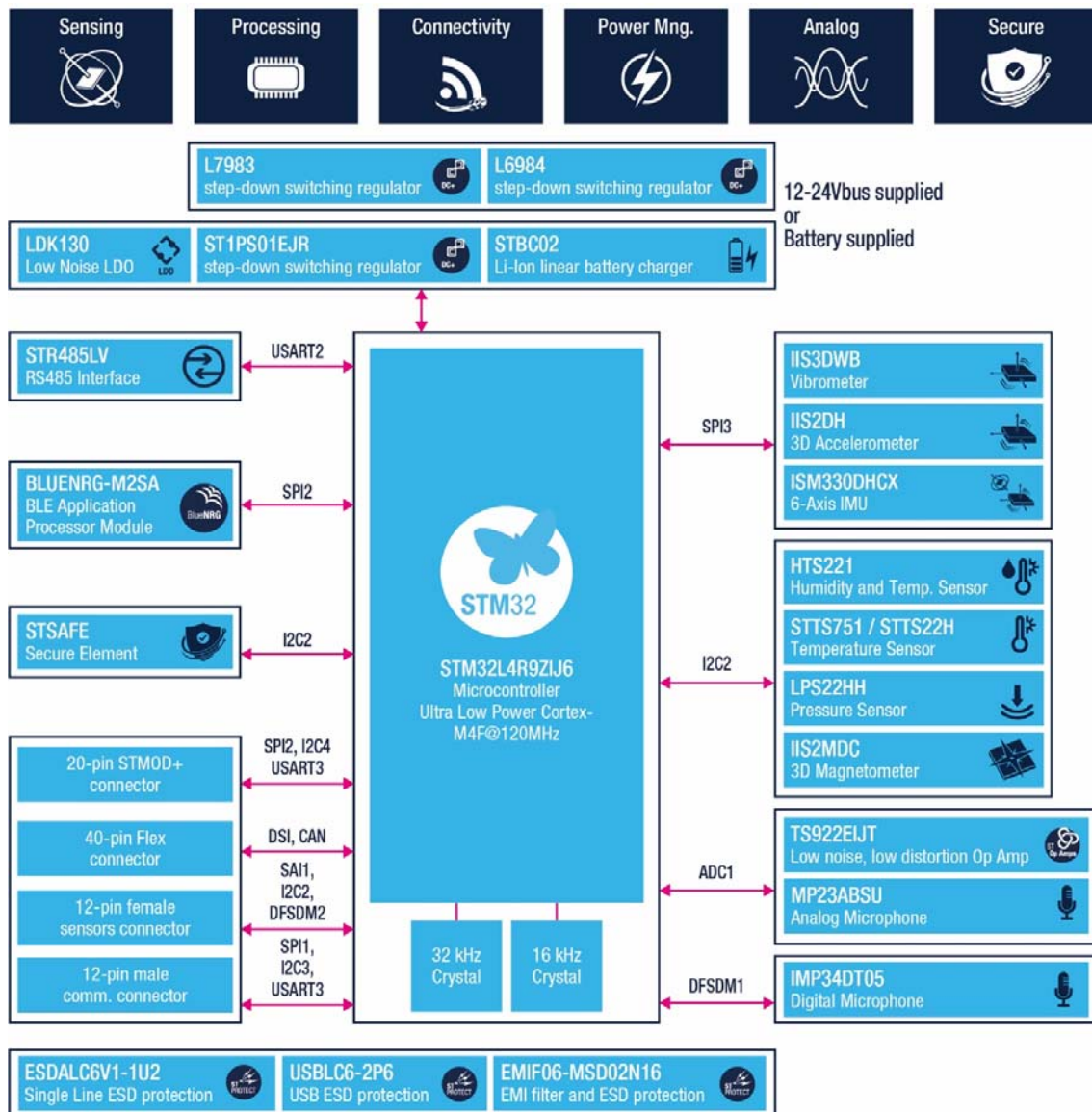
Fig. 1. Condition Monitoring turnkey solution
