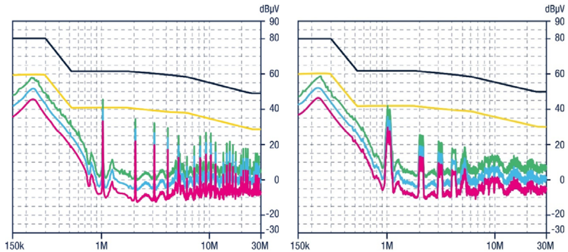
Fig. 3. V_{in} = 24V V_{out} = 3.3V , F_{sw} = 1 MHz, SS = OFF
