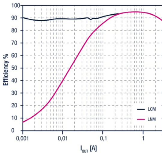
Fig. 9. V IN = 12V; V OUT 5V, LCM-LNM, F sw = 400 kHz
