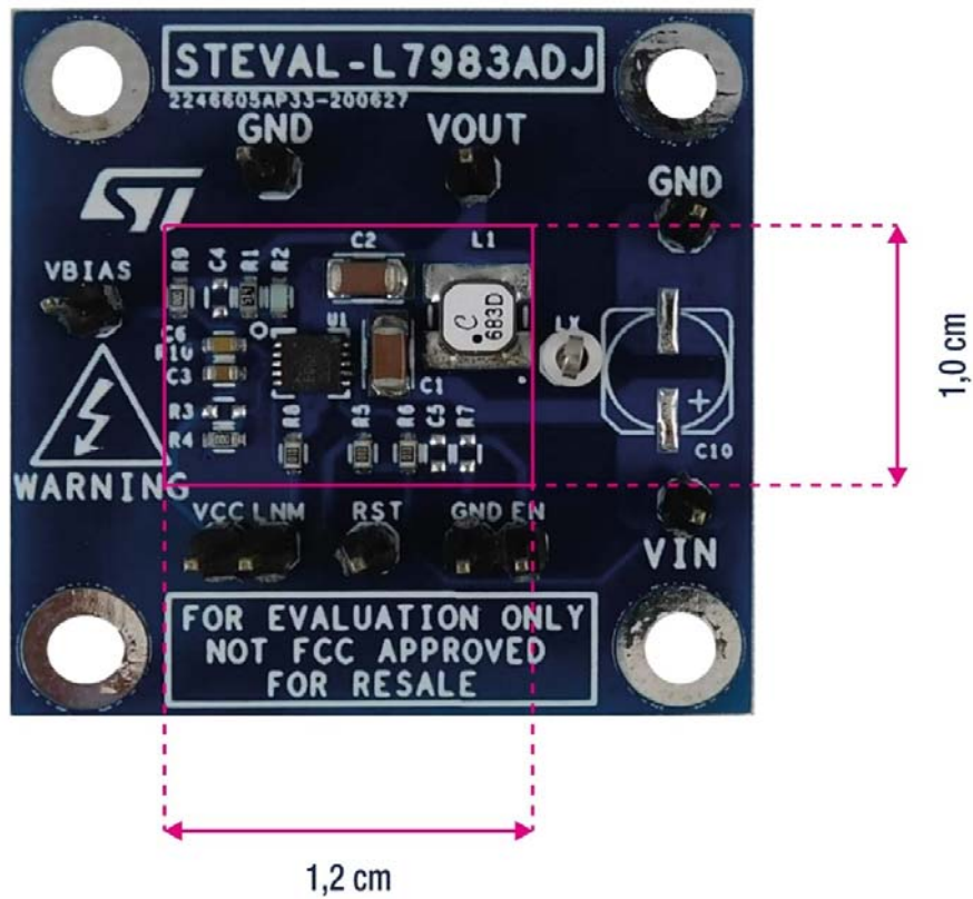
Fig. 7. L7983 Footprint
