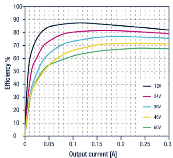
Fig. 6. Efficiency vs load, V_{out} = 3.3V , LNM, F_{sw} = 1 MHz
