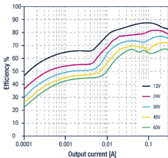
Fig. 5. Efficiency vs load, V_{out} = 3.3V , LCM, F_{sw} = 1 MHz
