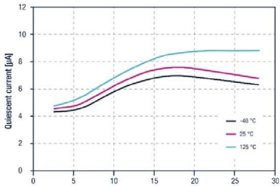
Fig. 8. ST73x family quiescent current vs V IN (@I OUT =0mA)
