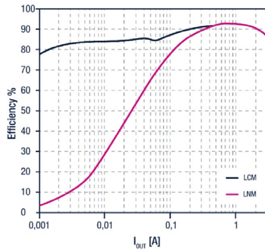
Fig. 10. V IN = 24V; V OUT 5V, LCM-LNM, F sw = 400 kHz
