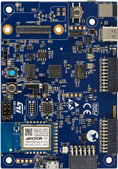
B-U585I-IOT02A top view. Picture is not contractual.
