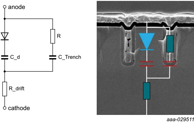
Figure 3: Equivalent circuit diagram of a Trench Schottky rectifier. The circuit elements are highlighted in the device cross section.
