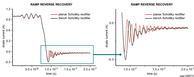
Figure 4: Ramp reverse recovery measurements on Trench and planar rectifiers. 100A/μs ramp
