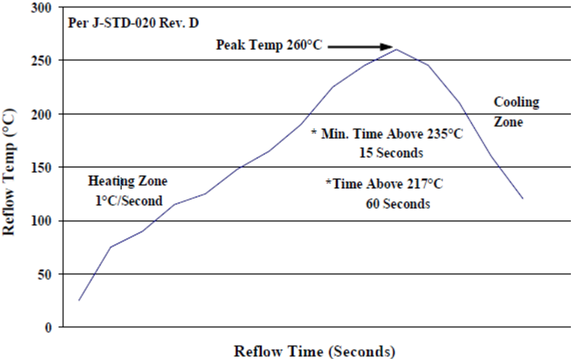
Figure 41. Recommended linear reflow profile using Sn/Ag/Cu solder
