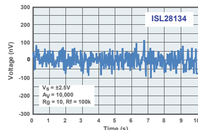
Figure 2. Input Noise Voltage 0.1Hz to 10Hz
