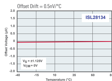
Figure 1. V_{OS} vs Temperature
