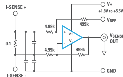
Bi-Directional Current Sense Amplifier
