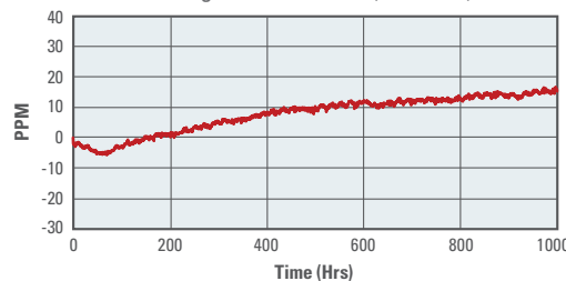
ISL21090 Long Term Drift Data (1000 Hrs)
