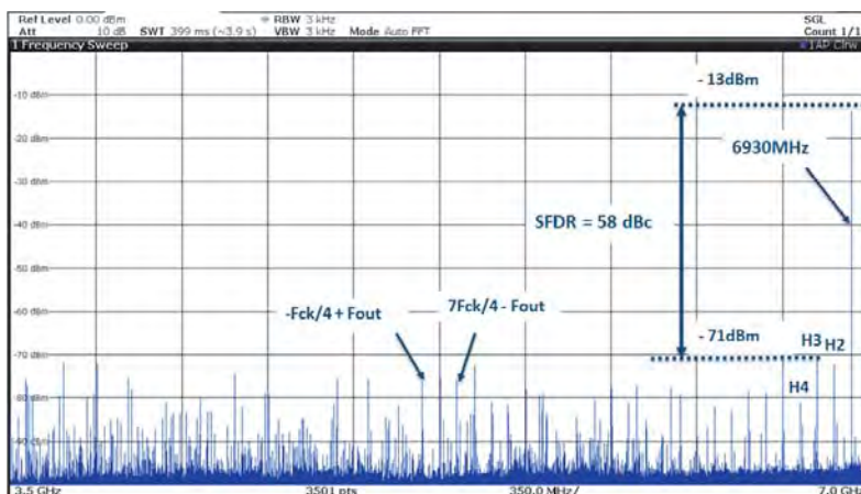
Figure 7-25. Typical SFDR spectrum in RF mode with F_{out} = 6930 MHz ( 2^{nd} Nyquist), MUX4:1, F_s = 7.0 GSps, SFDR = 58 dBc
