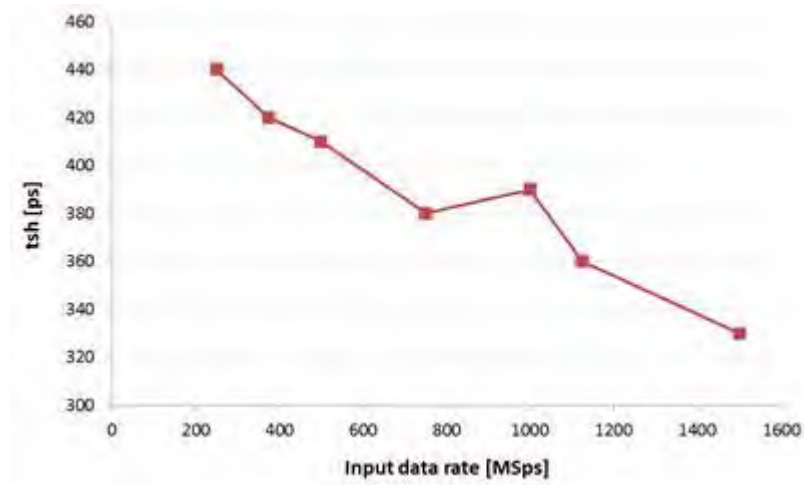
Figure 7-66. t_{SH} vs input data rate
