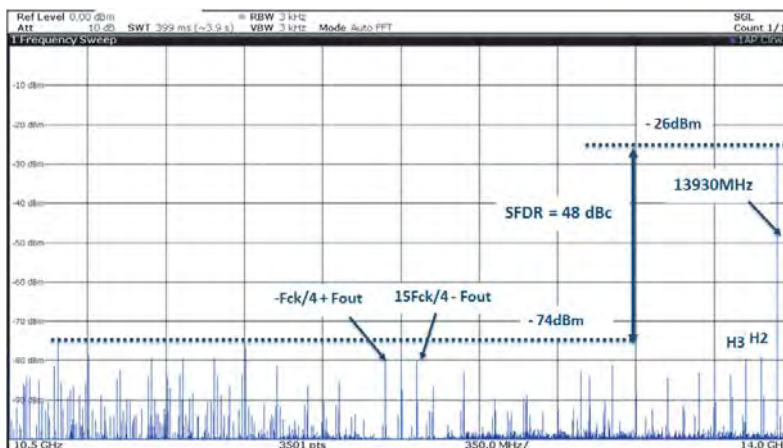
Figure 7-27. Typical SFDR spectrum in RF mode with F_{out} = 13930 MHz ( 4^{th} Nyquist), MUX4:1, F_s = 7.0 GSps, SFDR = 48 dBc
