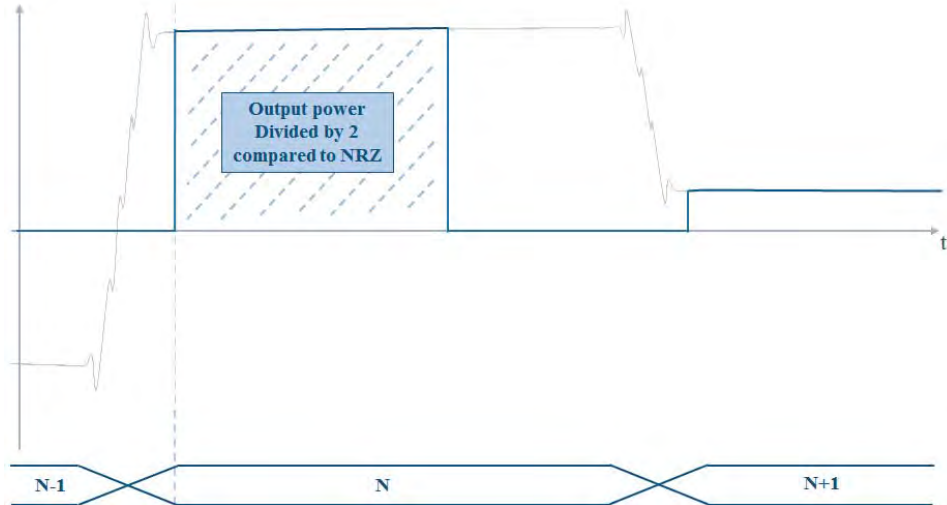
Figure 5-10. DAC output in RTZ mode and time domain when RPB is not optimum
