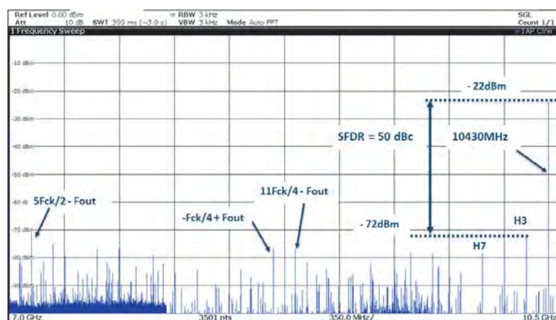
Figure 7-26. Typical SFDR spectrum in RF mode with F_{out} = 10430 MHz ( 3^{rd} Nyquist), MUX4:1, F_s = 7.0 GSps, SFDR = 50 dBc
