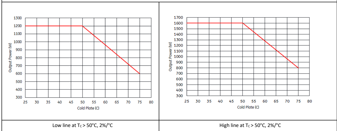
Output power derating curve with temperature
