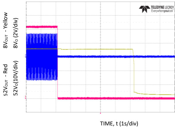
Figure 14. Turn-OFF at full load V_{IN} = 230V_{AC} .
