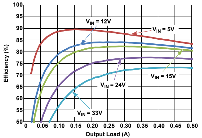
Figure 23. Efficiency vs Load, PMW, V_{OUT} = 1.8V
