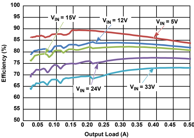
Figure 10. Efficiency vs Load, PFM, V_{OUT} = 1.8V
