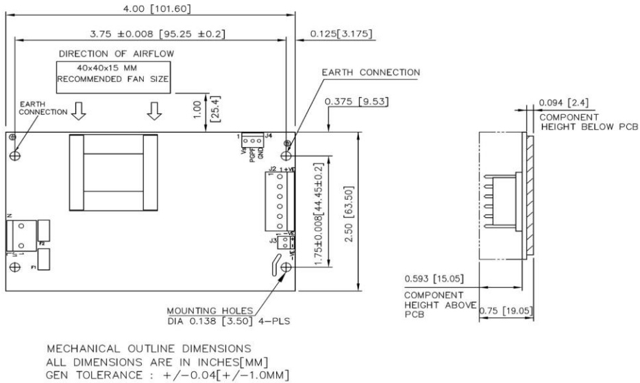
Mechanical Drawing – Option 2 with PGPF
