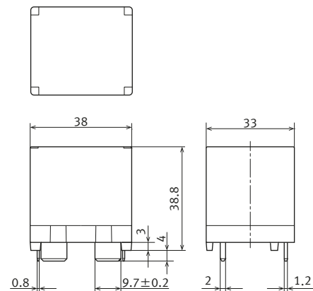
External dimensions
