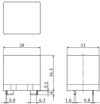
External dimensions
