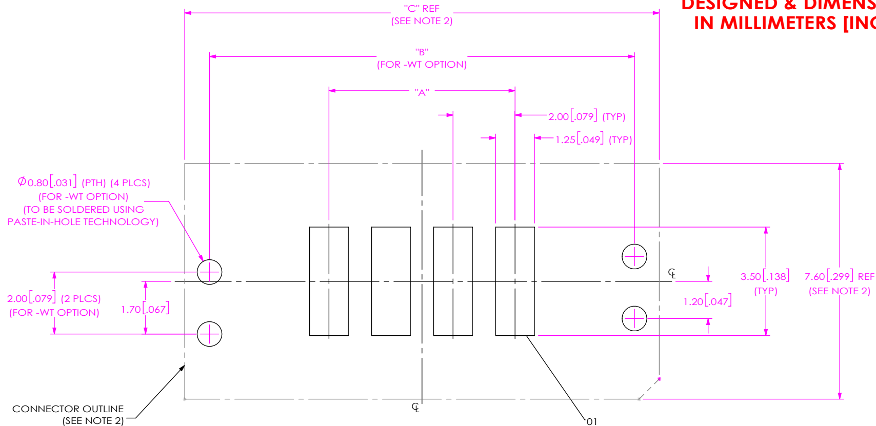
E UMPT-04-XX.X-XX-V-S-X-W-X-XR FOOTPRINT SHOWN
