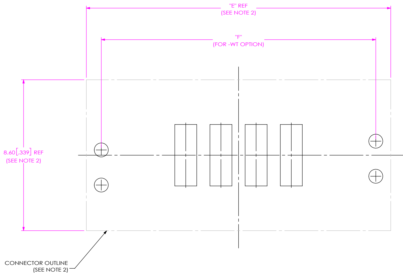
E FIG 5 UMPT-04-XX.X-XX-V-S-X-W-M-XR FOOTPRINT SHOWN (DIFFERENT AS SHOWN, OTHERWISE SAME AS FIG 1)
