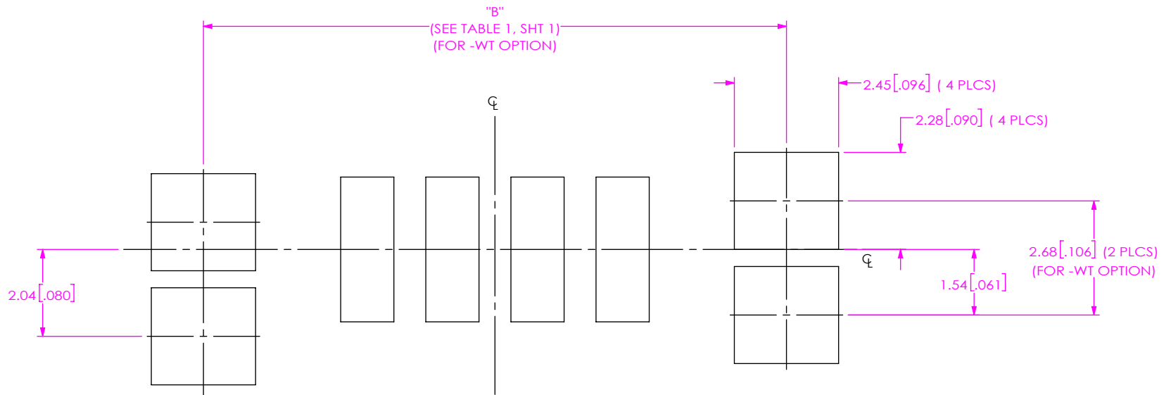
E FIG 2 UMPT-04-XX.X-XX-V-S-X-W-X-XR STENCIL SHOWN (DIFFERENT AS SHOWN, OTHERWISE SAME AS FIG 1)
