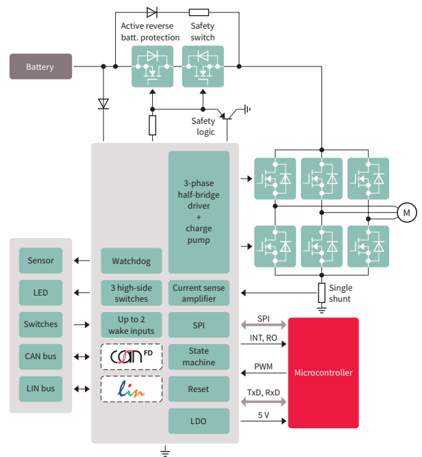
TLE9563/4 for BLDC motor control
