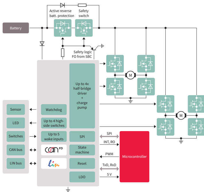
TLE9560/1/2 for DC motors control
