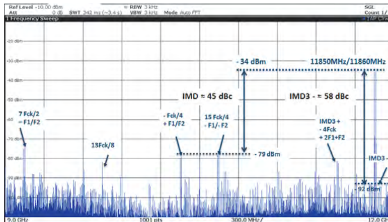
Figure 7-44. Typical Dual-tone spectrum in RF mode with F_{out1}, F_{out2} = 11850 \text{ MHz}, 11860 \text{ MHz} ( 4^{th} Nyquist), MUX4:1, F_s = 6.0 \text{ GSps} , \text{IMD3} = -58 \text{ dBc} , \text{IMD full Nyquist} = 45 \text{ dBc}
