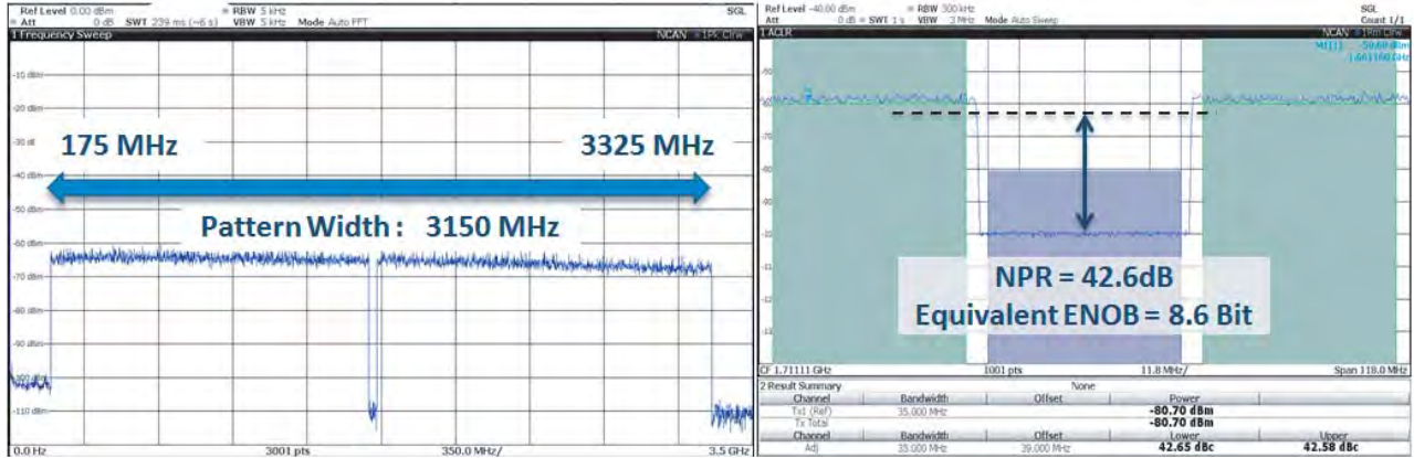
Figure 7-60. NPR @ 7.0 GSps in 1 st Nyquist, 3150 MHz pattern, NPR = 42.6 dB (= 8.6 Bit equivalent ENOB), NRTZ mode
