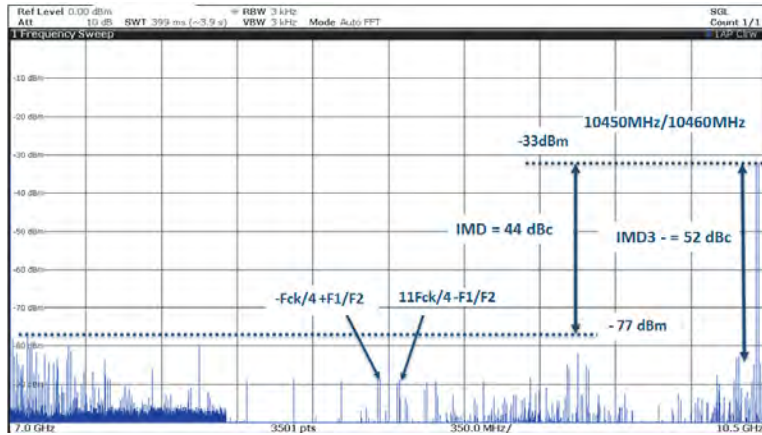
Figure 7-47. Typical Dual-tone spectrum in RF mode with F_{out1}, F_{out2} = 10450 \text{ MHz}, 10460 \text{ MHz} ( 3^{\text{rd}} Nyquist), MUX4:1, F_s = 7.0 \text{ GSps} , \text{IMD3} = -52 \text{ dBc} , \text{IMD full Nyquist} = 44 \text{ dBc}
