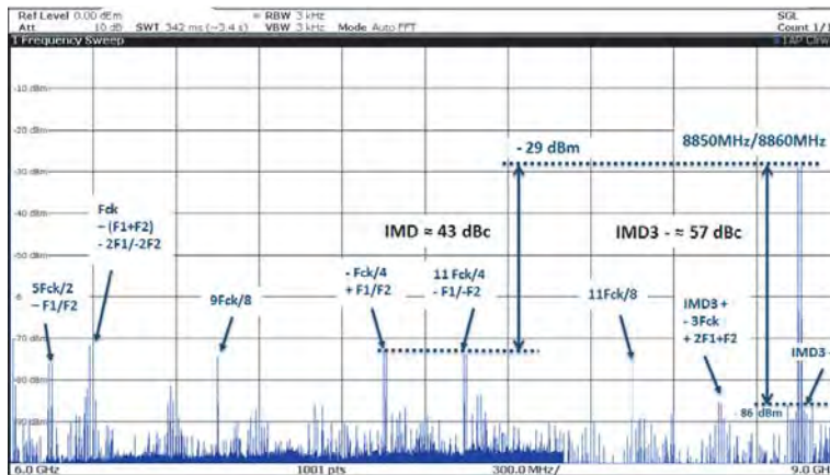
Figure 7-43. Typical Dual-tone spectrum in RF mode with F_{out1}, F_{out2} = 8850 \text{ MHz}, 8860 \text{ MHz} ( 3^{rd} Nyquist), MUX4:1, F_s = 6.0 \text{ GSps} , \text{IMD3} = -57 \text{ dBc} , \text{IMD full Nyquist} = 43 \text{ dBc}
