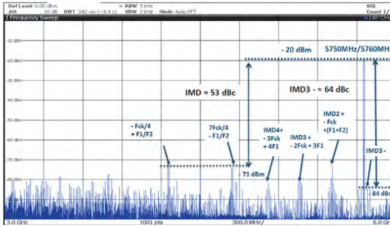
Figure 7-42. Typical Dual-tone spectrum in RF mode with F_{out1}, F_{out2} = 5750 \text{ MHz}, 5760 \text{ MHz} , ( 2^{nd} Nyquist), MUX4:1, F_s = 6.0 \text{ GSps} , \text{IMD3} = -64 \text{ dBc} , \text{IMD full Nyquist} = 53 \text{ dBc}
