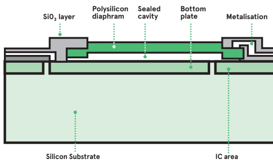
▲ A cross section of a capacitive MEMS sensor construction
