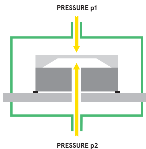
▲ Differential pressure measurement principle
