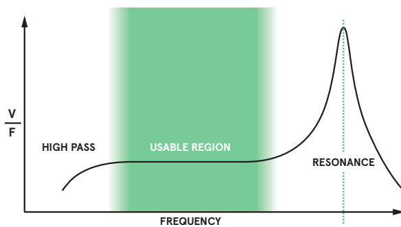
▲ The frequency response of a piezoelectric sensor
