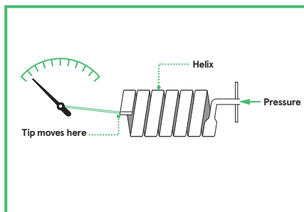
▲ Helical Bourdon tube
