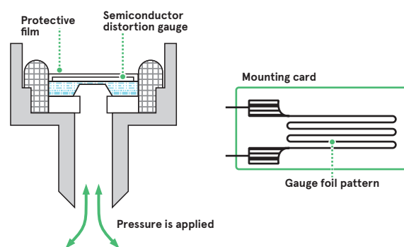
▲ The cross-section of a semiconductor distortion gauge, as used in many gas pressure sensors.
