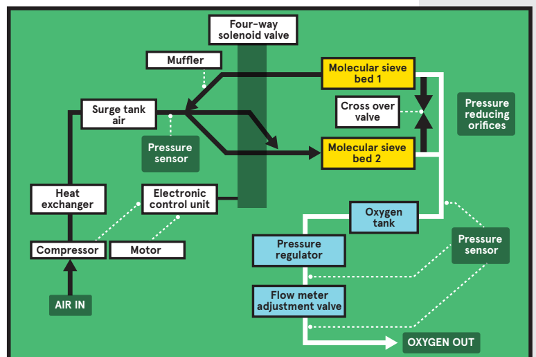
▲ Pressures sensors in an oxygen concentrator (Source: All Sensors)
