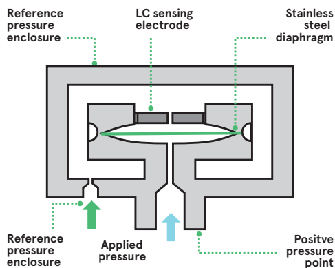
▲ A capacitive air pressure sensor
