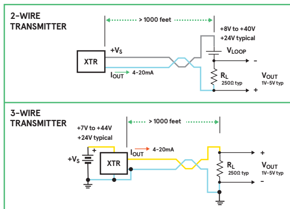
▲ Example circuits showing how a gauge sensor transmitter may be implemented
