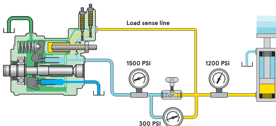
▲ A load-sensing hydraulic system featuring three pressure sensors
