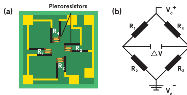
▲ Two ways in which piezoresistive elements might be arranged
