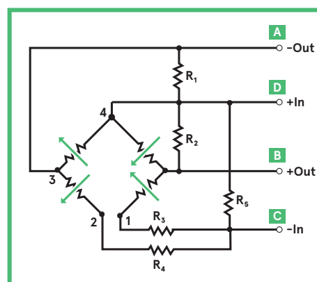
▲ Wheatstone bridge structure of an absolute pressure sensor
