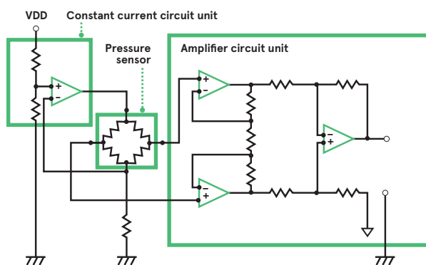
▲ A piezoresistive Wheatstone bridge circuit with amplifier, powered by a constant current circuit
