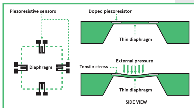
▲ Piezo resistive pressure sensor operating principle
