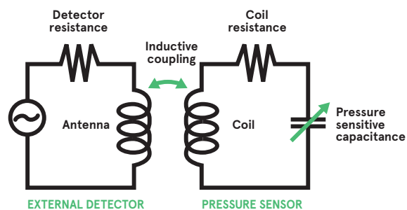
▲ An external antenna in some passive sensors to stimulate the tuned circuit
