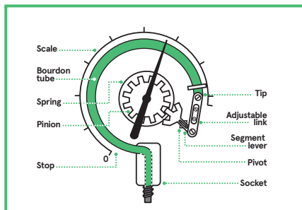
▲ C-shaped Bourdon tube
