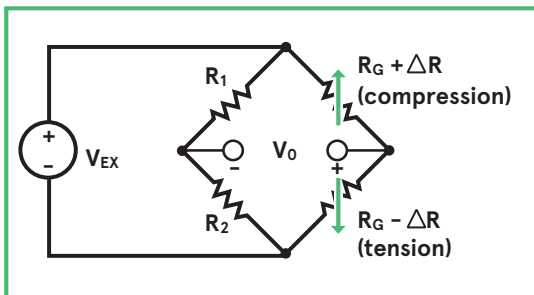
▲ A half-bridge strain gauge with millivolt output.
