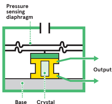
▲ The piezo electric effect can be exploited in multiple ways to sense pressure
