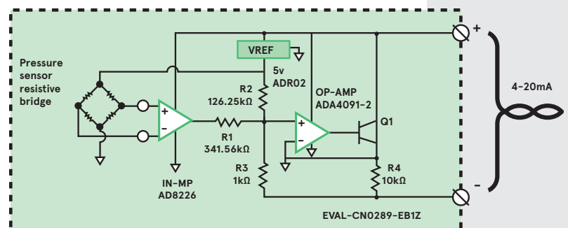
▲ A bridge-type sensor with transmitter output circuitry for an industrial 4–20mA application
