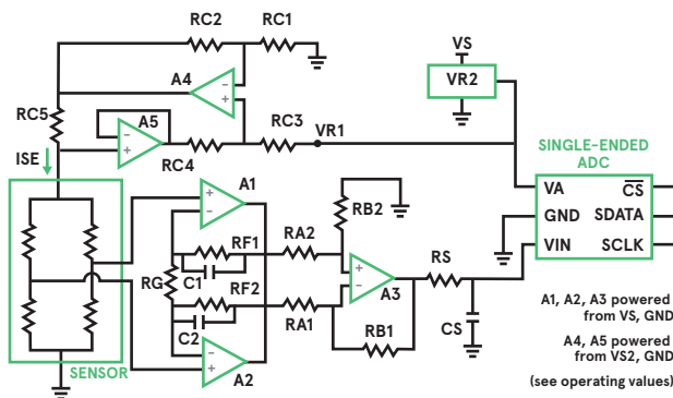
▲ An example circuit for amplifying the signal from a Wheatstone bridge piezoresistive pressure sensor.
