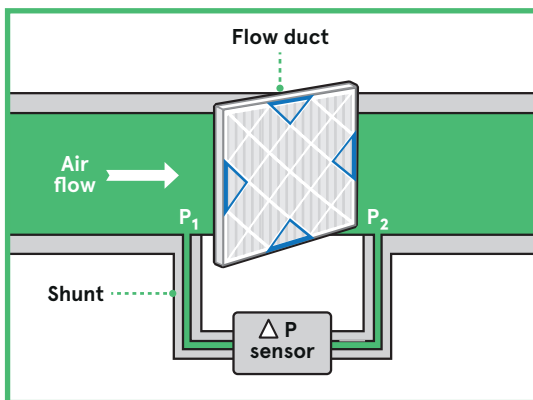
▲ A differential pressure sensor measuring the airflow through a filter
