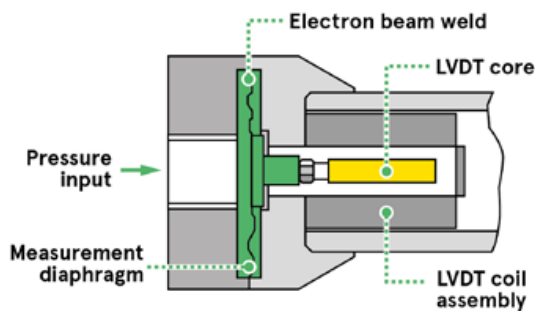
▲ A cross-section of a linear variable differential transformer pressure sensor
