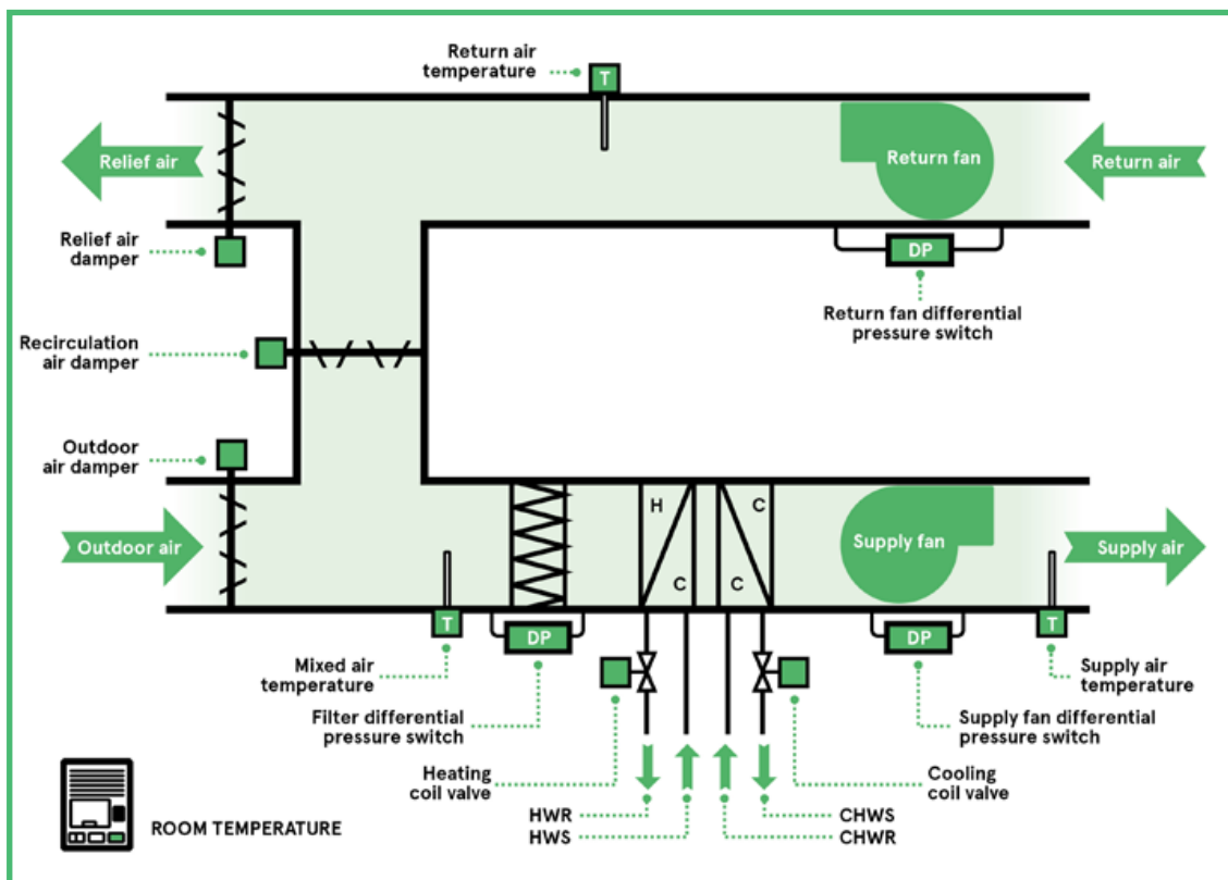
▲ A general representation of an HVAC system
