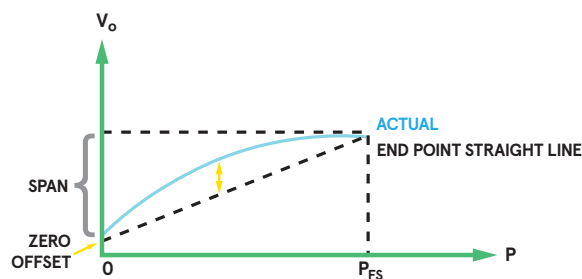
▲ Terminal line method for calculating non-linearity.
