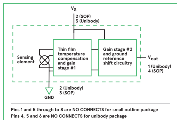
▲ Some analog sensors provide a considerable amount of analog circuitry around the sensing element
