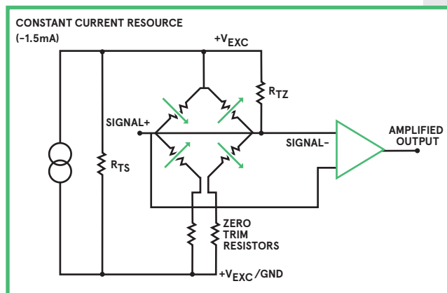
▲ Bridge-sensor circuit diagram
