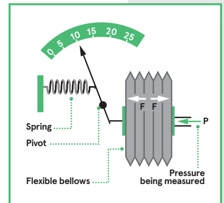
▲ The bellows operating principle
