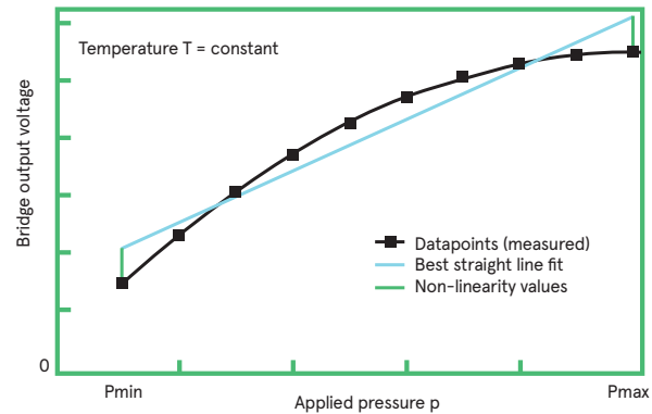
▲ A graphical representation of non-linearity using the Best Fit Straight Line method.
