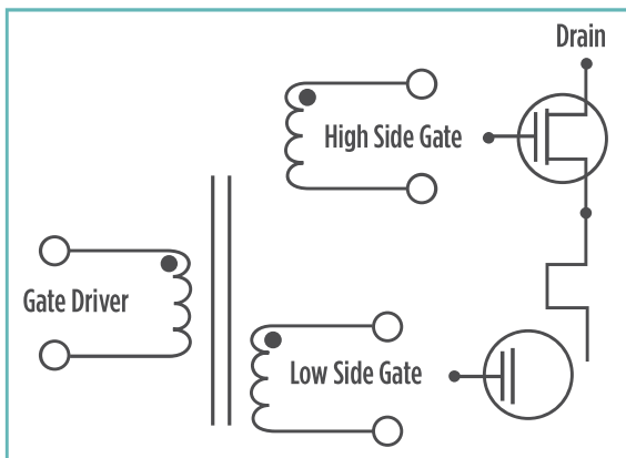
High Side, Low Side H-Bridge
