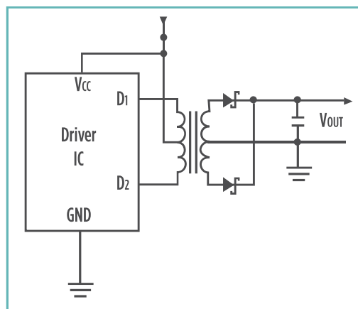
Push-pull Isolation Transformer
