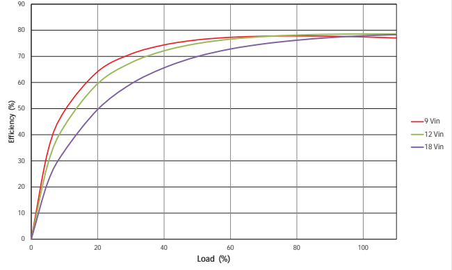
MTC1S1205SC
