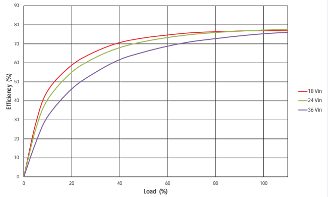
MTC1S2412SC
