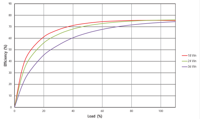
MTC1S2403SC
