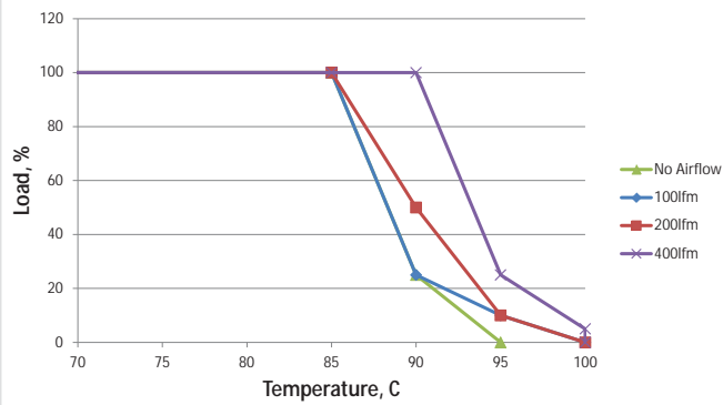
MTC1S1212SC - 18Vin
