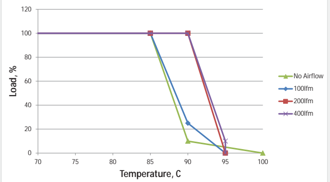
MTC1S2403SC - 36Vin
