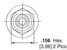
Straight Bulkhead Jack' Part Number 141-1001-0001 Instruction Sheet Number 408-8512 Former MICRODOT I.S. Number RF-ASMB-15
