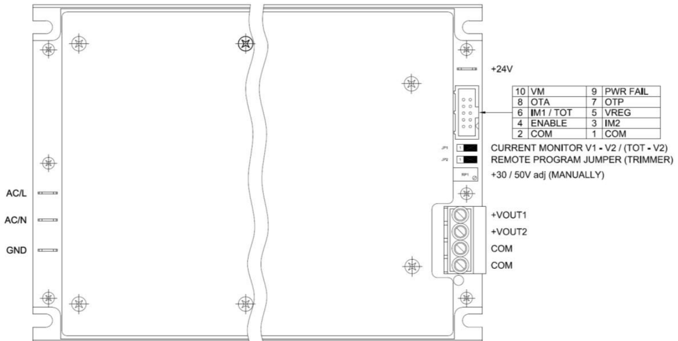
Figure 1 – Connections
