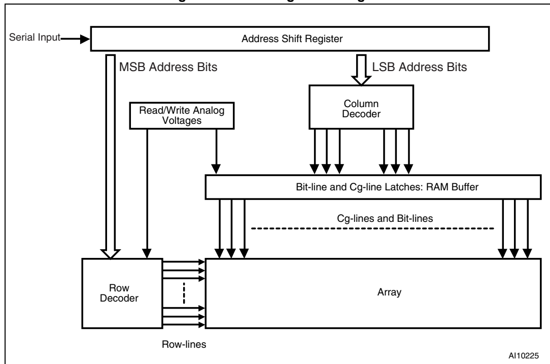
Figure 11. Decoding block diagram
