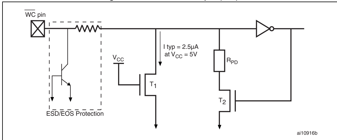
Figure 20. Write control input ( \overline{WC} )
