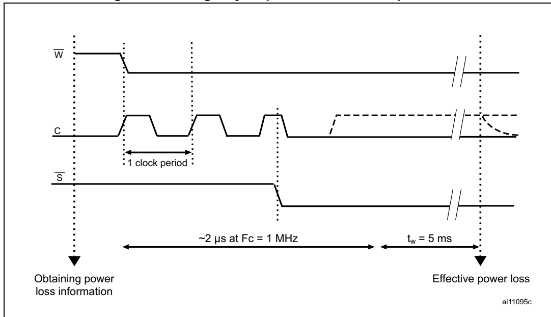
Figure 46. Emergency sequence MICROWIRE products
