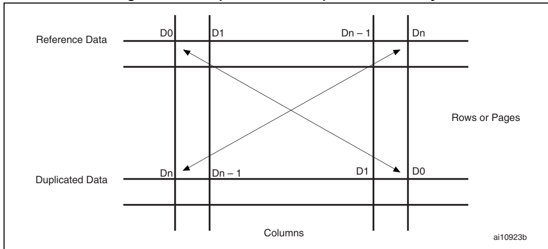
Figure 38. Example of how to duplicate data safely
