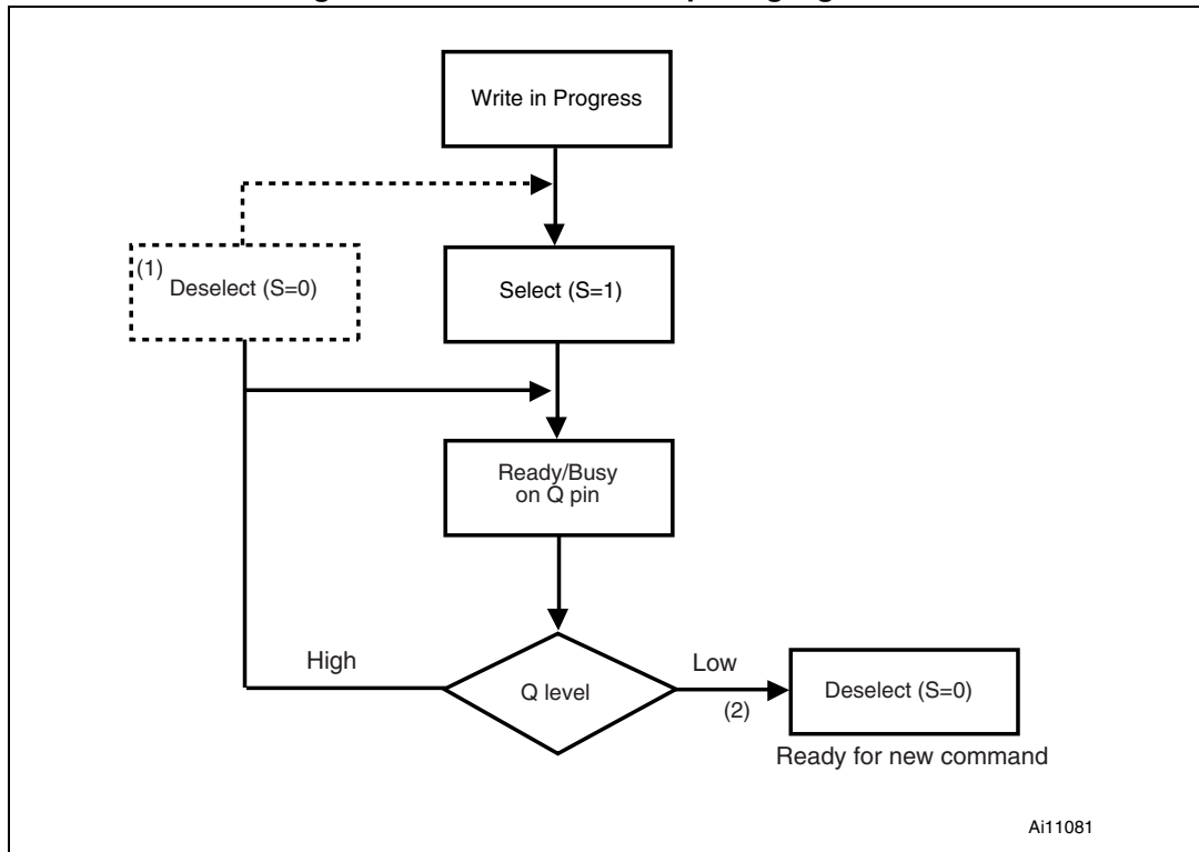
Figure 35. MICROWIRE data polling algorithm
