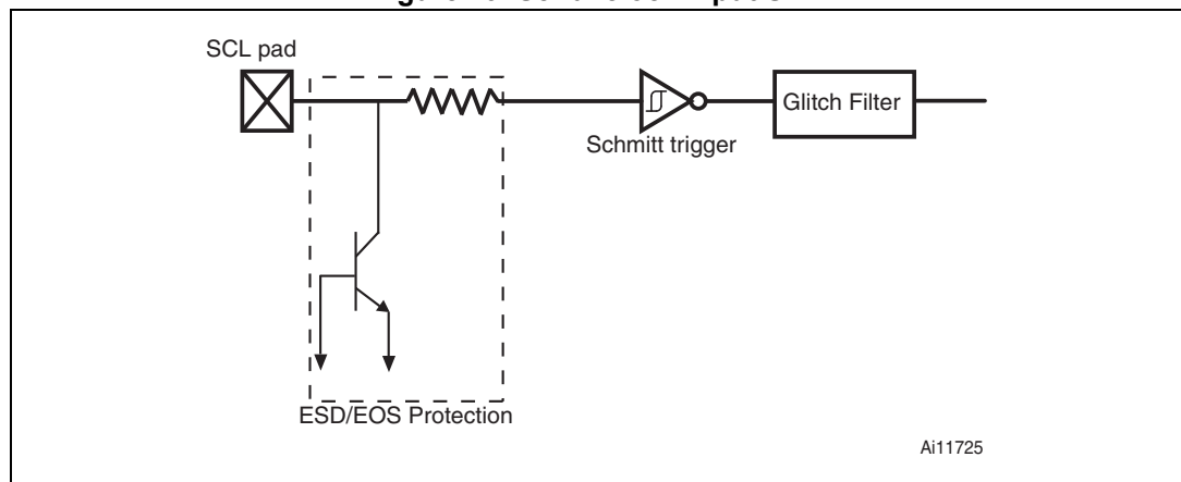
Figure 19. Serial clock input SCL
