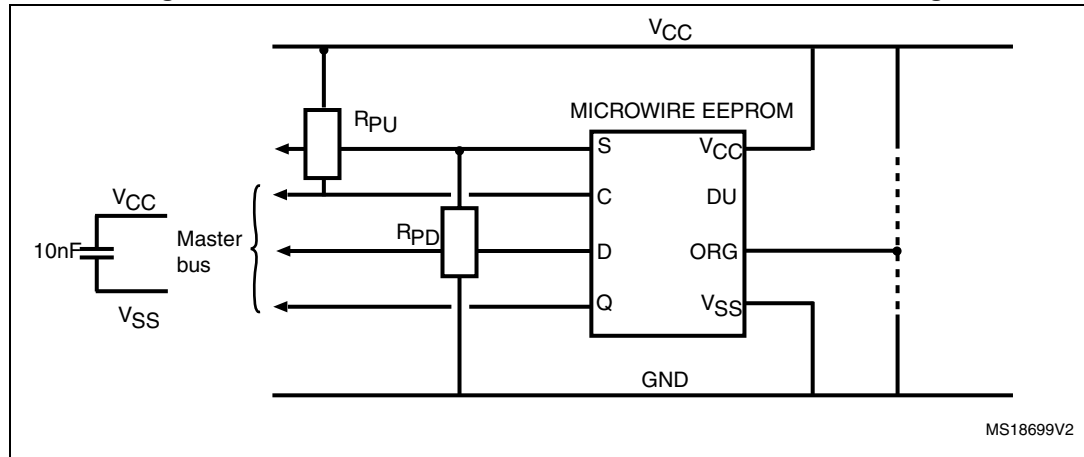
Figure 30. Recommended MICROWIRE connections - safe design
