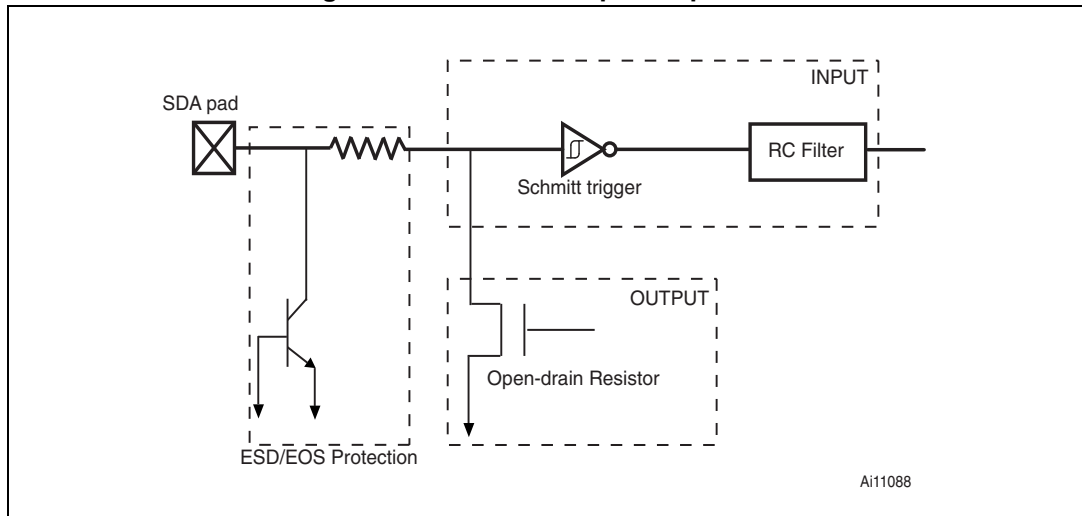
Figure 17. Serial Data input/output SDA
