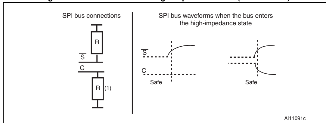
Figure 41. SPI bus enters the high impedance state (Master reset)
