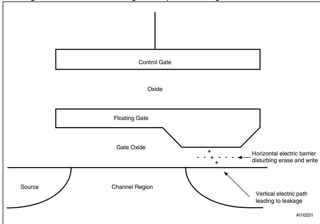
Figure 9. Accumulation of negative or positive charges in the tunnel oxide
