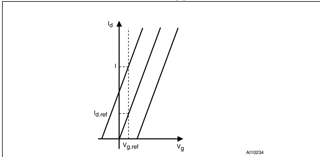
Figure 5. Using the voltage on the Control Gate to determine the charge on the floating gate
