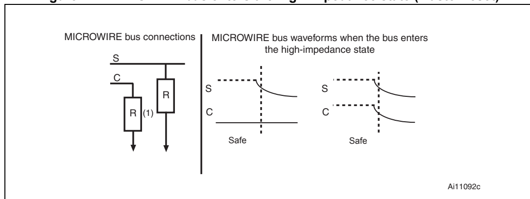
Figure 42. MICROWIRE bus enters the high impedance state (Master reset)
