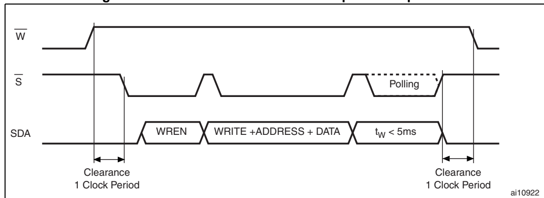
Figure 37. Recommended use of the \overline{W} pin in SPI products
