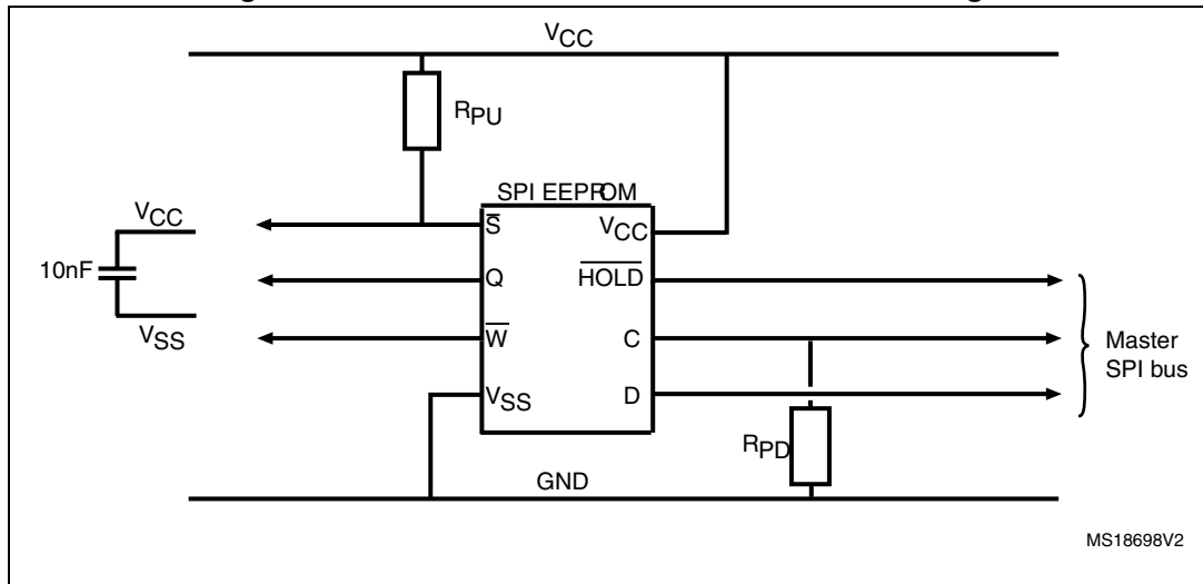
Figure 27. Recommended SPI connections - robust design
