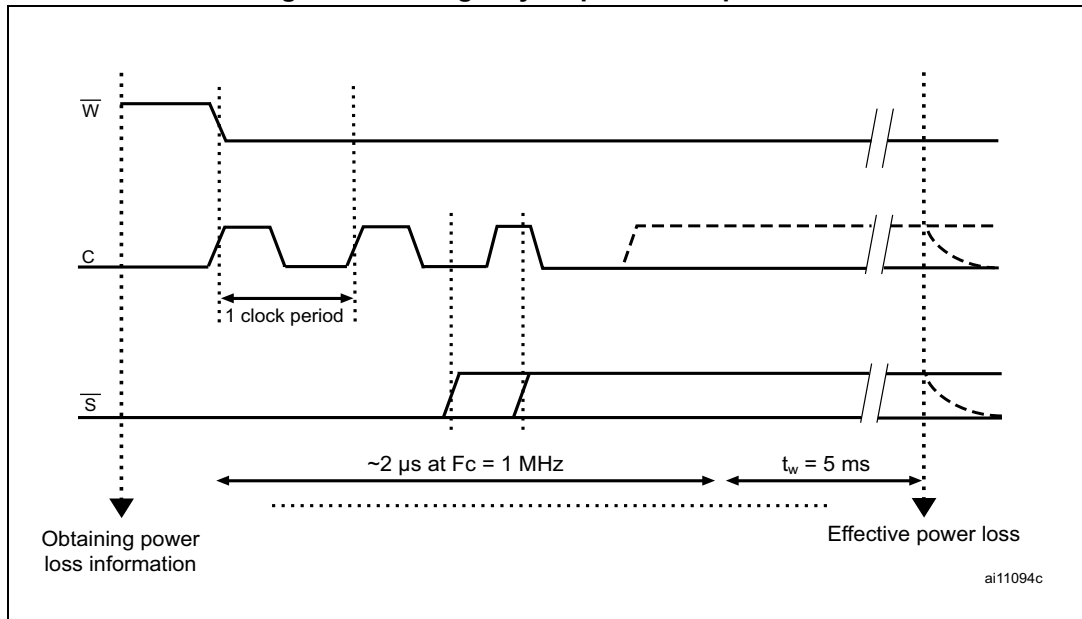
Figure 45. Emergency sequence SPI products
