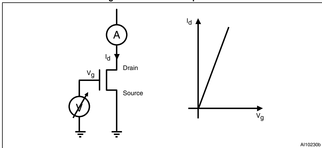
Figure 2. MOSFET-like operation
