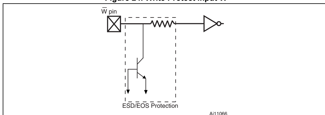
Figure 24. Write Protect input \overline{W}
