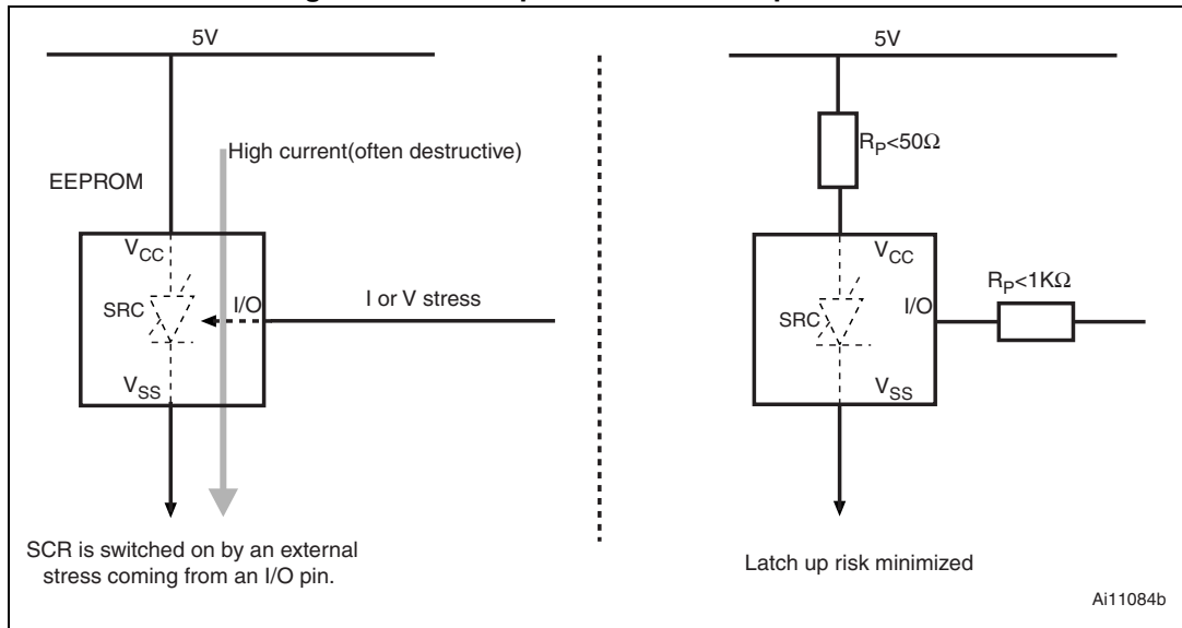
Figure 12. Latchup mechanism and protection
