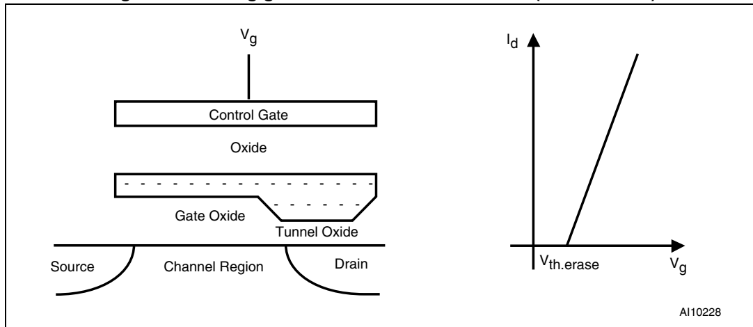
Figure 3. Floating gate reservoir full of electrons (Erased state)
