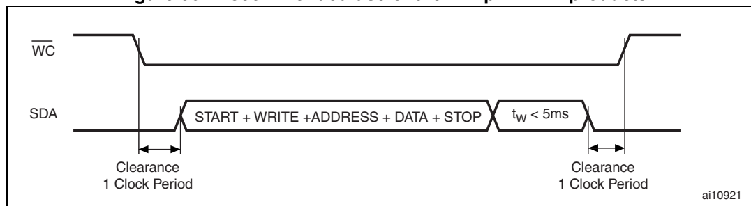
Figure 36. Recommended use of the \overline{WC} pin in I 2 C products
