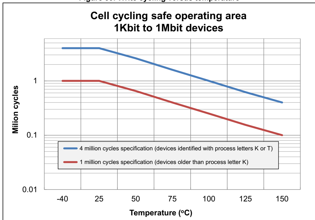
Figure 39. Write cycling versus temperature
