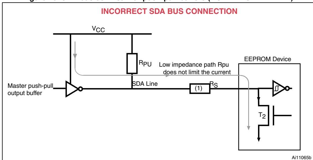
Figure 18. SDA bus conflict with push-pull buffers (NOT RECOMMENDED)
