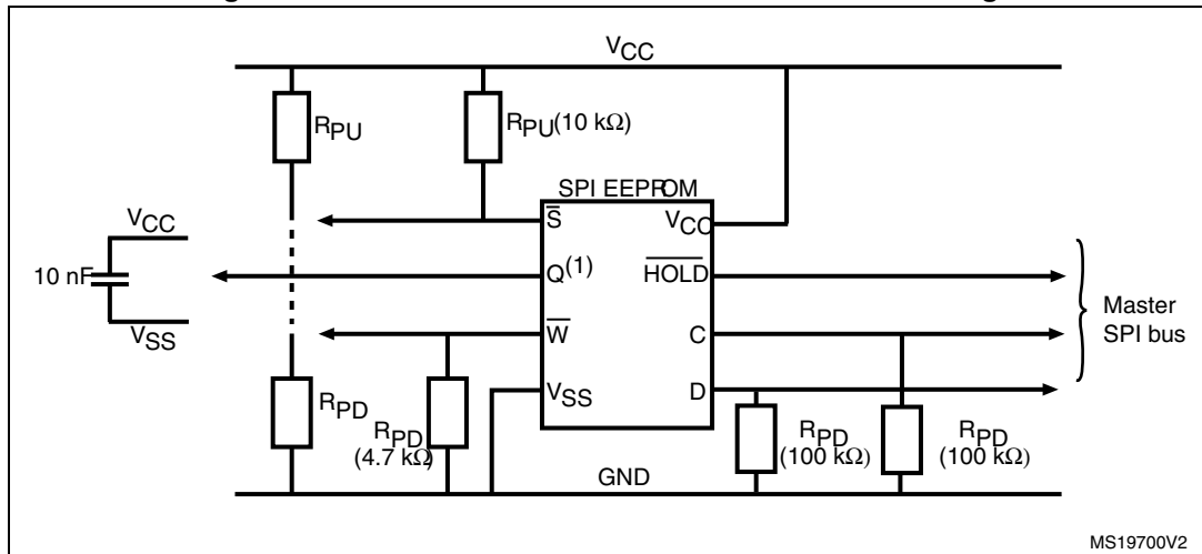
Figure 27. Recommended SPI connections - robust design
