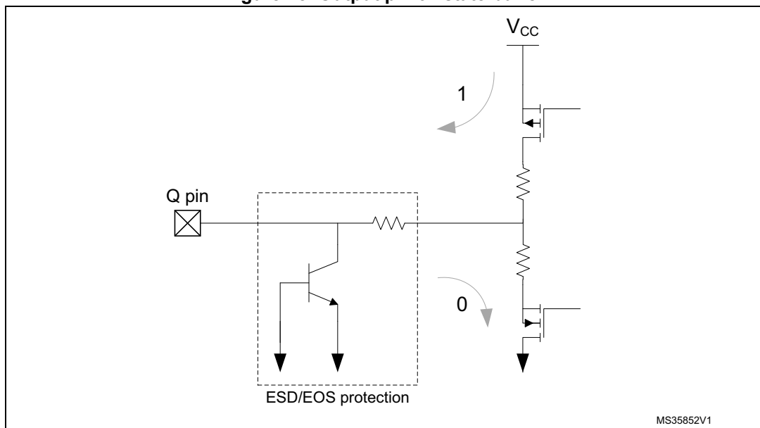
Figure 25. Output pin tri-state buffer
