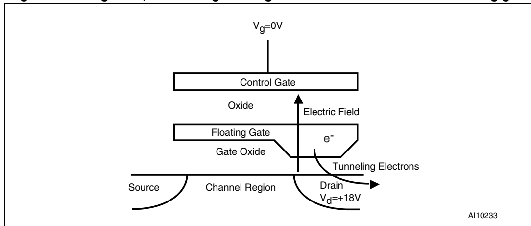
Figure 7. During write, electrons go through the tunnel oxide out of the floating gate
