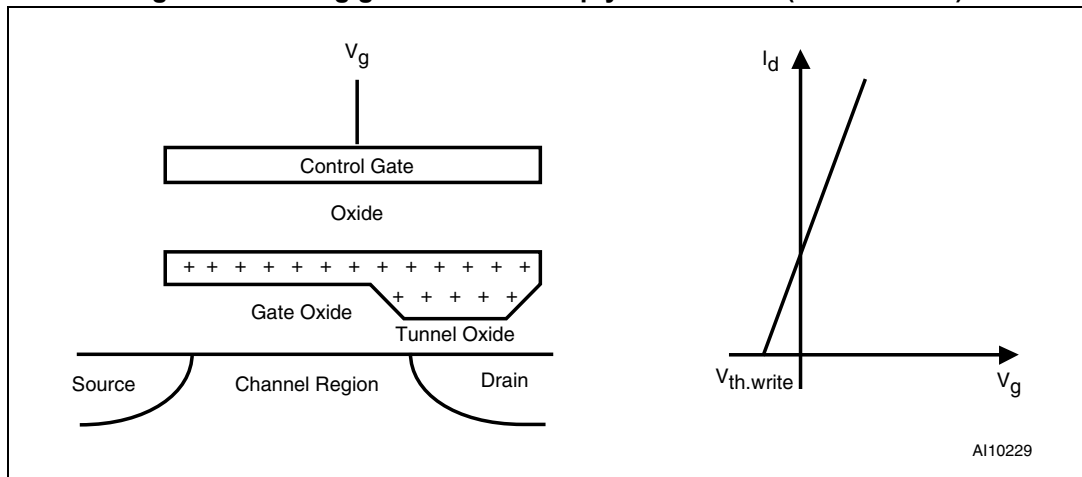
Figure 4. Floating gate reservoir empty of electrons (Written state)
