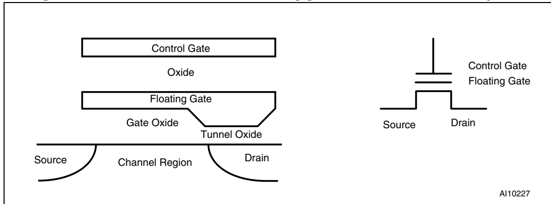
Figure 1. Structure of an EEPROM floating gate transistor, and circuit symbol
