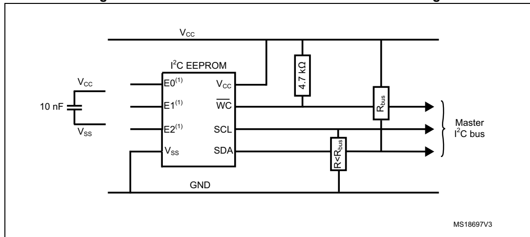
Figure 22. Recommended I 2 C connections – robust design
