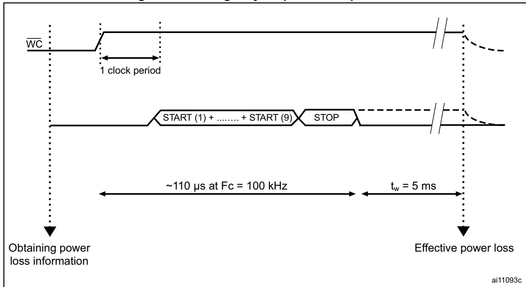
Figure 44. Emergency sequence I 2 C products
