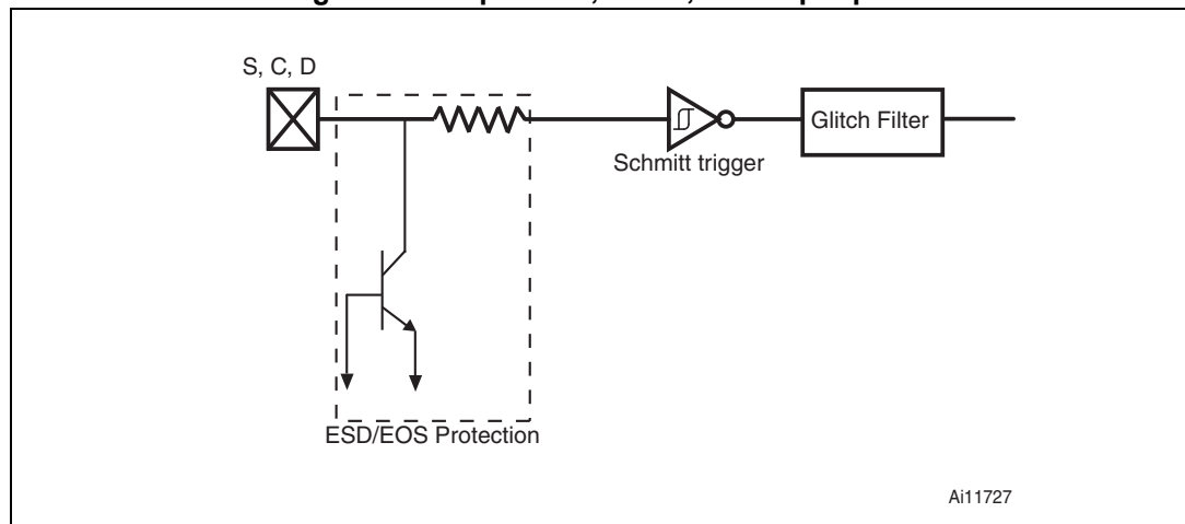
Figure 28. Chip Select, Clock, Data input pins
