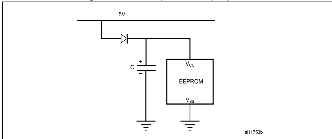
Figure 43. EEPROM power backup capacitor
