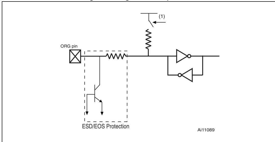
Figure 29. Organization input ORG
