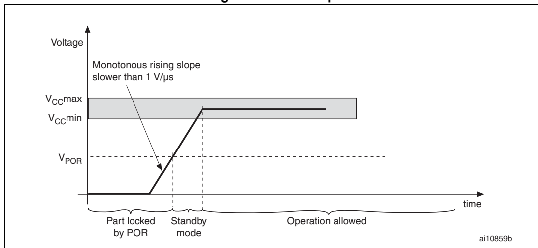
Figure 14. Power-up
