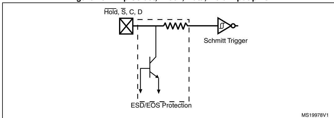
Figure 23. Chip Select, Clock, Data, Hold input pins
