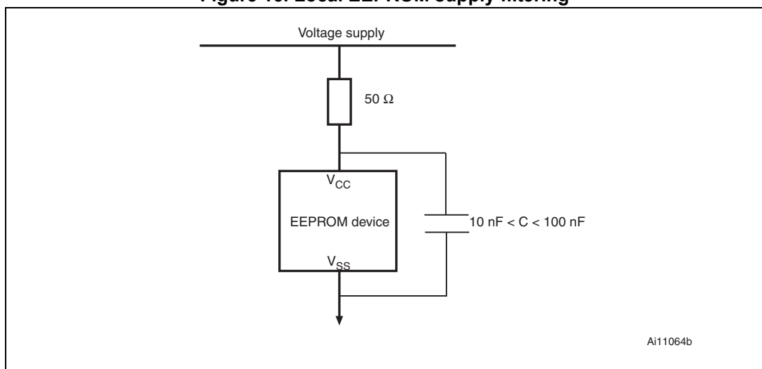
Figure 15. Local EEPROM supply filtering
