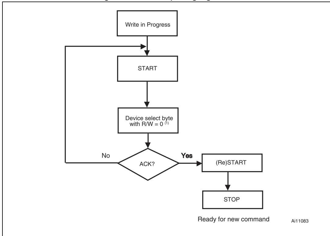
Figure 33. I 2 C data polling algorithm
