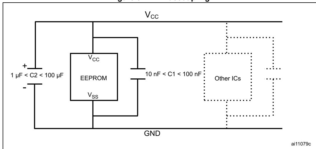
Figure 32. PCB decoupling
