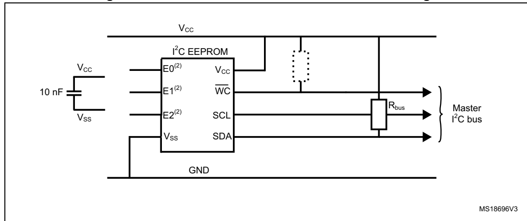
Figure 21. Recommended I 2 C connections – safe design
