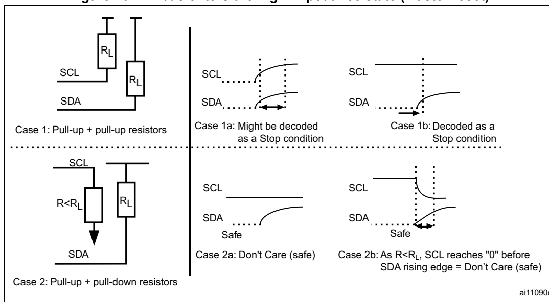
Figure 40. I 2 C bus enters the high impedance state (Master reset)
