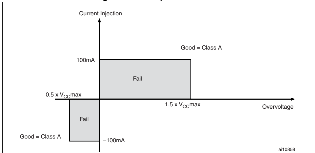
Figure 13. Latchup test conditions
