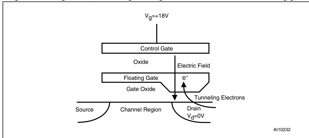
Figure 6. During erase, electrons go through the tunnel oxide into the floating gate
