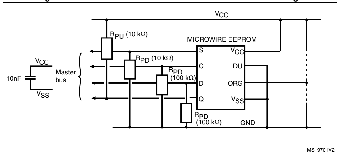
Figure 31. Recommended MICROWIRE connections - robust design
