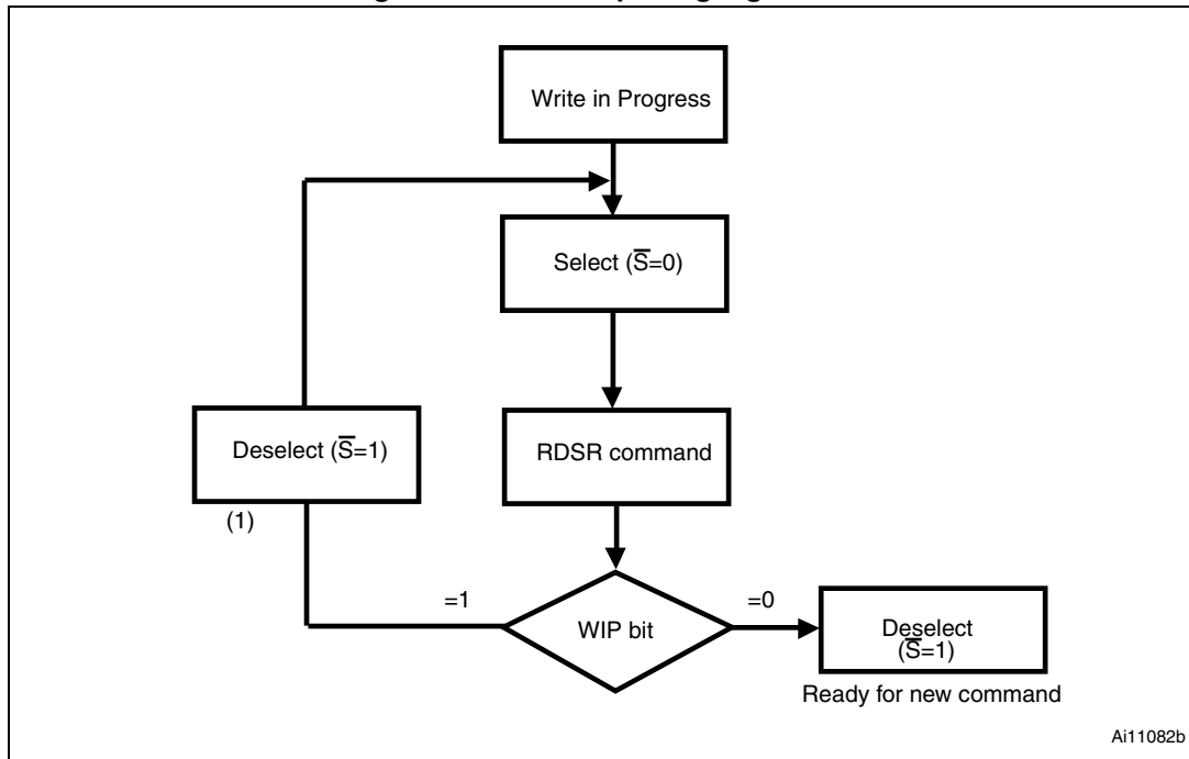
Figure 34. SPI data polling algorithm
