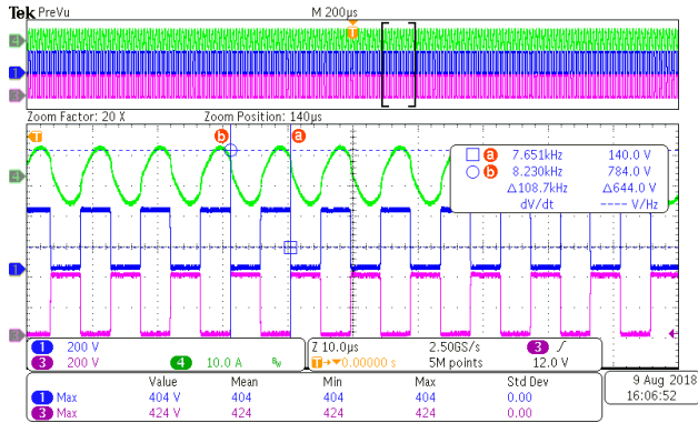
Figure 25. Vo = 400 Vdc, Load = 75%
