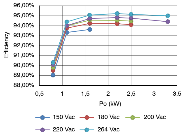
Figure 18. Efficiency vs. Po Curve @ Vo = 380 Vdc
