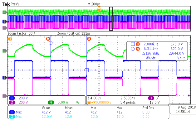
Figure 23. Vo = 400 Vdc, Load = 25%
