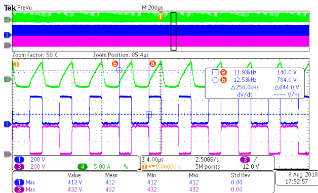
Figure 28. Vo = 350 Vdc, Load = 25%
