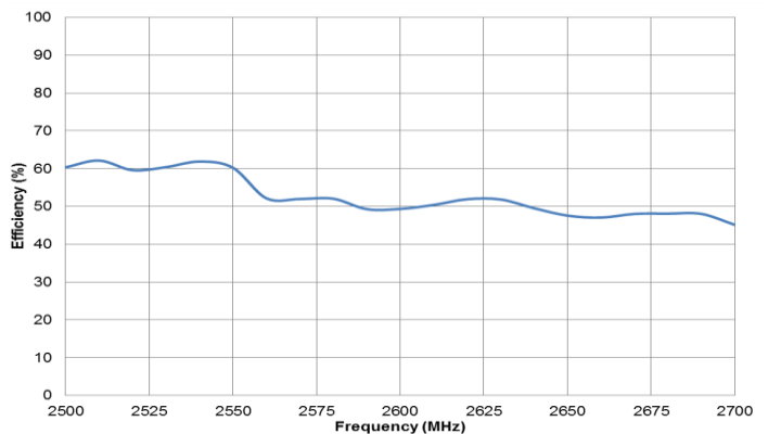
Band 7 Efficiency
