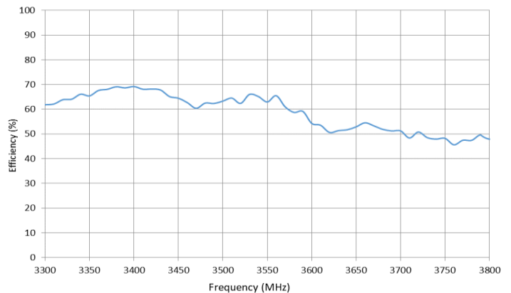
n78 Efficiency
