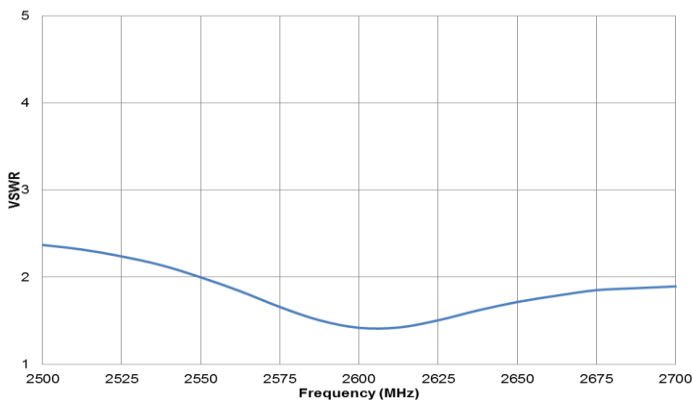
Band 7 VSWR
