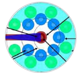
Launch Optimization
