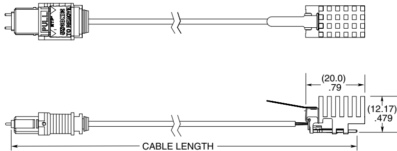
PCUO-04-G4-XXX-0-4-1-8-01 SHOWN
