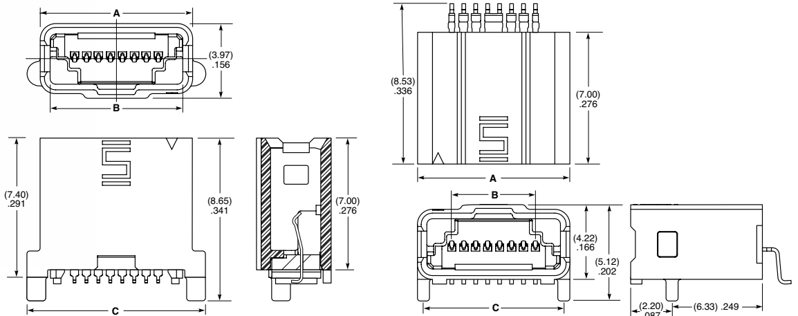
AMF6-02-S-K-XR SHOWN
