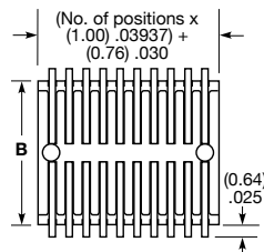
-06 & -10 Contact Detail
