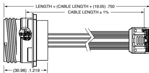
NVA3P-DP-1-19-XX.X-A-X-1-Z-S SHOWN
