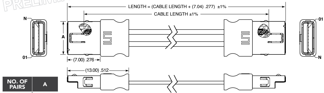
ARM6-02-XX.X-LU-LU-4-X SHOWN
