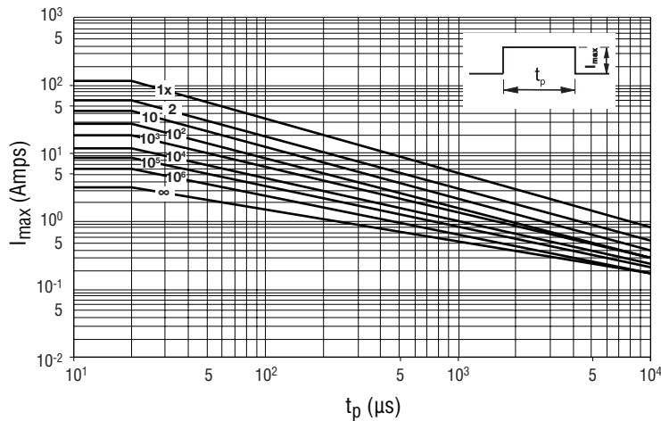
Model Size 1206 - (ZV 35 K 1206 121 HT ~ ZV 60 K 1206 121 HT)
