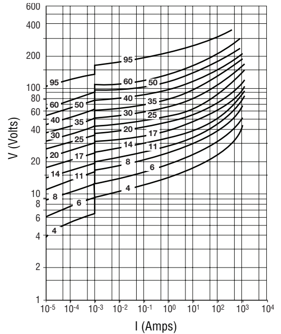
Model Size 2220 - (ZV 4 M 2220 xxx HT ~ ZV 95 K 1210 xxx HT)
