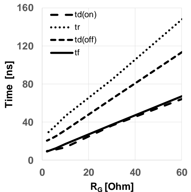
Figure 18 Typical switching times as a function of gate resistor ( t = f(R_{G,ext}) , V_{DD} = 800V , V_{GS} = 0V/18V , I_D = 16A , T_{vj} = 175^\circ C , ind. load, test circuit in Fig. E, diode: body diode at V_{GS} = 0V )
