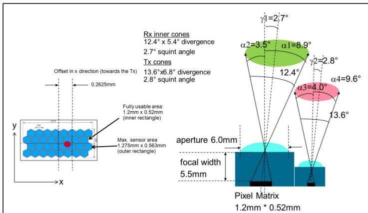
Figure 6: Field-of-View (FoV) Description of the Sensor
