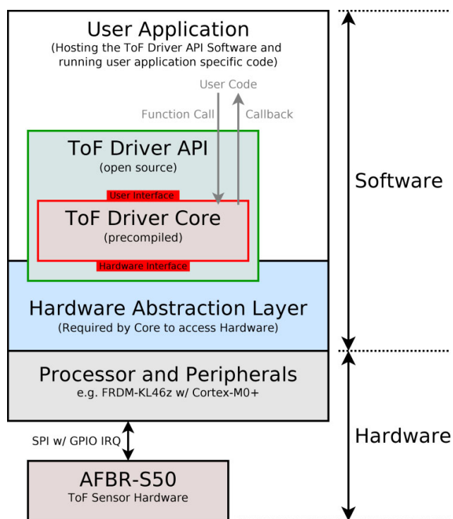
Figure 13: Driver Software Block Diagram
