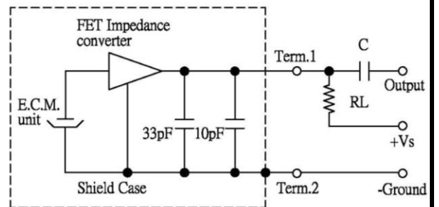
Schematic Diagram
