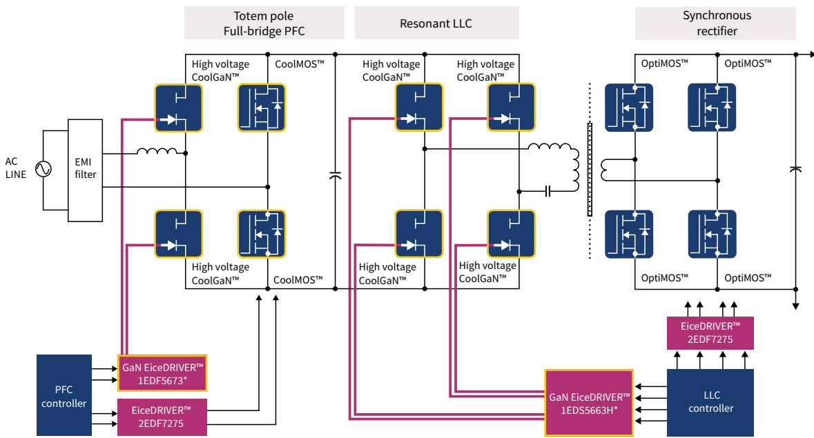
*GaN EiceDRIVER™ ICs are single-channel products
