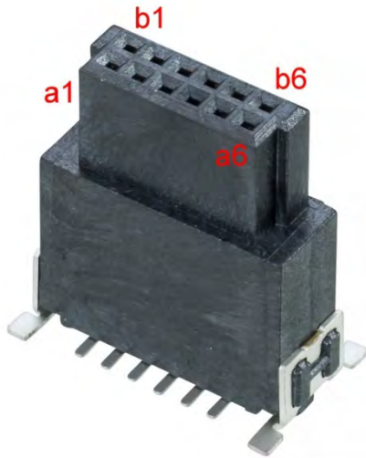
Female Connectors
